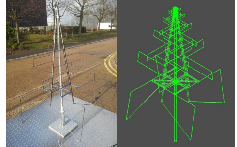
Fig. 1. The SKALA antenna outside the Cavendish Laboratory, Cambridge (left) and a computer model of the antenna used for the EM simulations (right).
