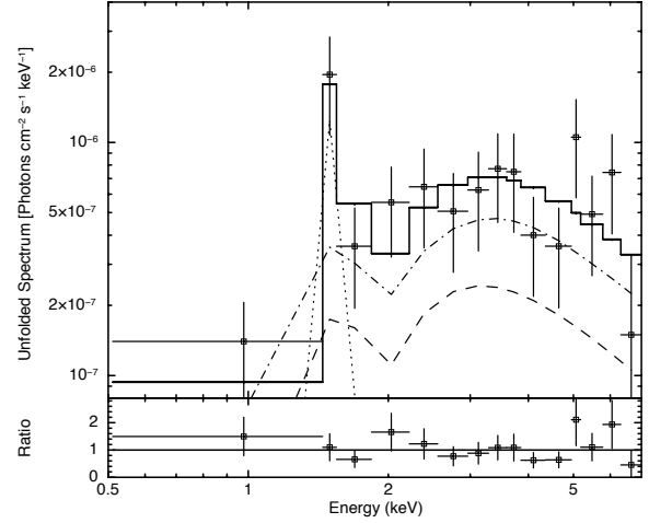
Figure 1. Upper panel: unfolded X-ray spectrum of W0116–0505, rebinned ( 2\sigma per bin) for display purposes, and total best-fitting model (solid line). The transmitted component (i.e., absorbed power-law), scattered continuum, and iron K\alpha emission-line component are shown as dashed, dot-dashed, and dotted lines, respectively. Lower panel: ratio between the data points and the model expectations. The best-fitting MYTorus model is consistent with being Compton thick.
