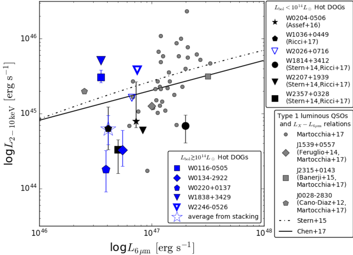
Figure 5. Intrinsic X-ray luminosity versus mid-IR luminosity for Hot DOGs. Blue and black symbols represent individual sources presented in this work or collected from the literature. See Appendix A for the analysis on W2026+0716. Error bars are given at 68% confidence level. Downward pointing arrows represent upper limits on the X-ray luminosities at 90% confidence level. The average X-ray luminosity for stacked sources (derived from Fig. 4 assuming a column density of N_H = 10^{24} \text{ cm}^{-2} ) is marked at their median L_{6\mu m} with a blue star. We also add for comparison the sample of luminous optical Type 1 QSOs collected by Martocchia et al. (2017), and we plot the relations of Stern (2015) and Chen et al. (2017).
