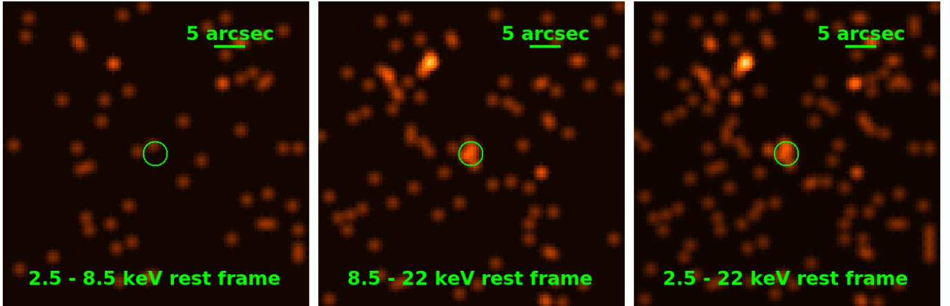
Figure 2. From left to right: stacked and smoothed X-ray images in the rest-frame 2.5 – 8.5, 8.5 – 22.0, and 2.5 – 22.0 keV bands. Each panel has a dimension of 101 \times 101 pixels (about 50 \times 50 arcsec). Solid circles have radii of 4 pixels ( \approx 2 arcsec) and represent the extraction regions we used to compute the photometry. The significant emission in the upper central parts of the images (especially in the hard and full bands) is due to a serendipitously detected X-ray source (with 7–9 counts) in the proximity ( \approx 16 arcsec offset) of W2246–7143.
