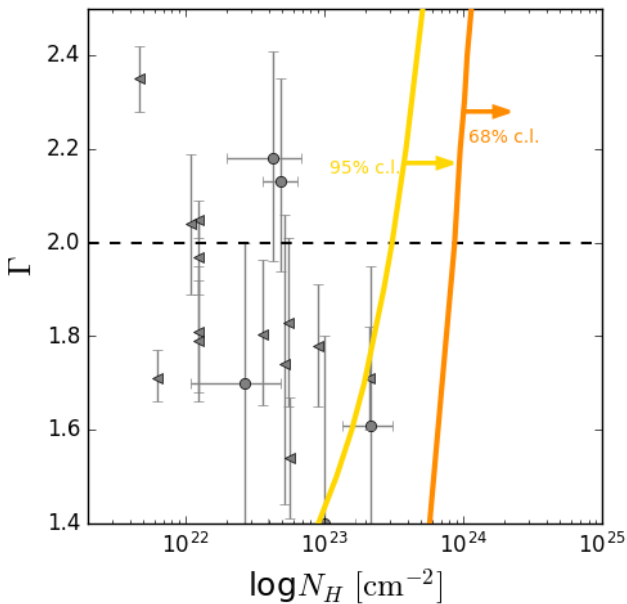
Figure 3. Confidence limits (at 68% and 95% levels, in orange and gold, respectively) in the \Gamma - N_H plane obtained from hardness-ratio analysis of the stacked emission of our sample. Grey symbols are from the sample of optical Type 1 QSOs from Martocchia et al. (2017). Leftward-pointing symbols are upper limits (90% confidence level) on column density. The dashed horizontal line represents the value for \Gamma we assumed in § 5.1.
