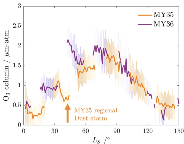
Figure 10. Averaged UVIS O_3 columns between 20^\circ S and 20^\circ N as a function of L_S for the aphelion season in MY 35 (orange line) and MY 36 (purple line). The vertical lines give the 1-\sigma dispersion of the data.
