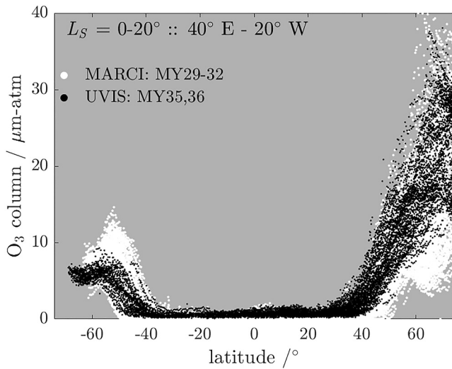
Figure 4. A comparison of ozone column latitudinal dependence retrieved by UVIS in MY 35 and MY 36 against those by MARCI for MY29-32 (Clancy et al., 2016) over the period L_S = 0^\circ – 20^\circ and between 40^\circ E– 20^\circ W.
