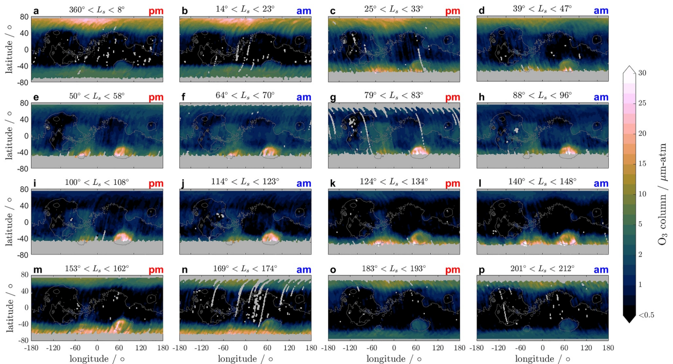
Figure 7. The geographical distribution of ozone for MY 35 between L_S = 0 – 212^\circ . Each panel alternates between the afternoon and morning atmosphere that is, panels (a, c, e, g, i, k, m, o), represent local solar times between 1200 LST and 1800 LST and panels (b, d, f, h, j, l, n, p) present the morning retrievals from 0600 LST to 1200 LST. The irregular L_S periods and the gaps in L_S are due to the orbital coverage and the beta angle causing no observations, respectively. Note the color scale in non-linear to highlight lower O_3 columns.
