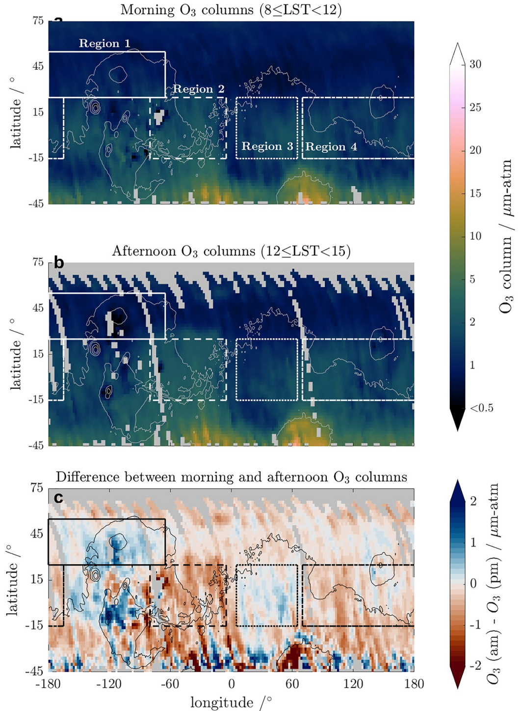
Figure 14. The UVIS O 3 column abundances as a function of latitude and longitude between L_S = 79.5 – 90.5 in MY 35 for (a) The morning between 8 \leq \text{LST} < 12\text{LST} and (b) the afternoon 12 \leq \text{LST} < 15 . (c) The difference between the morning and afternoon O 3 column abundances (am–pm). The four different regions investigated are outlined in (c) by a solid line (Region 1), dash line (Region 2), dotted line (Region 3), and dash-dot line (Region 4).
