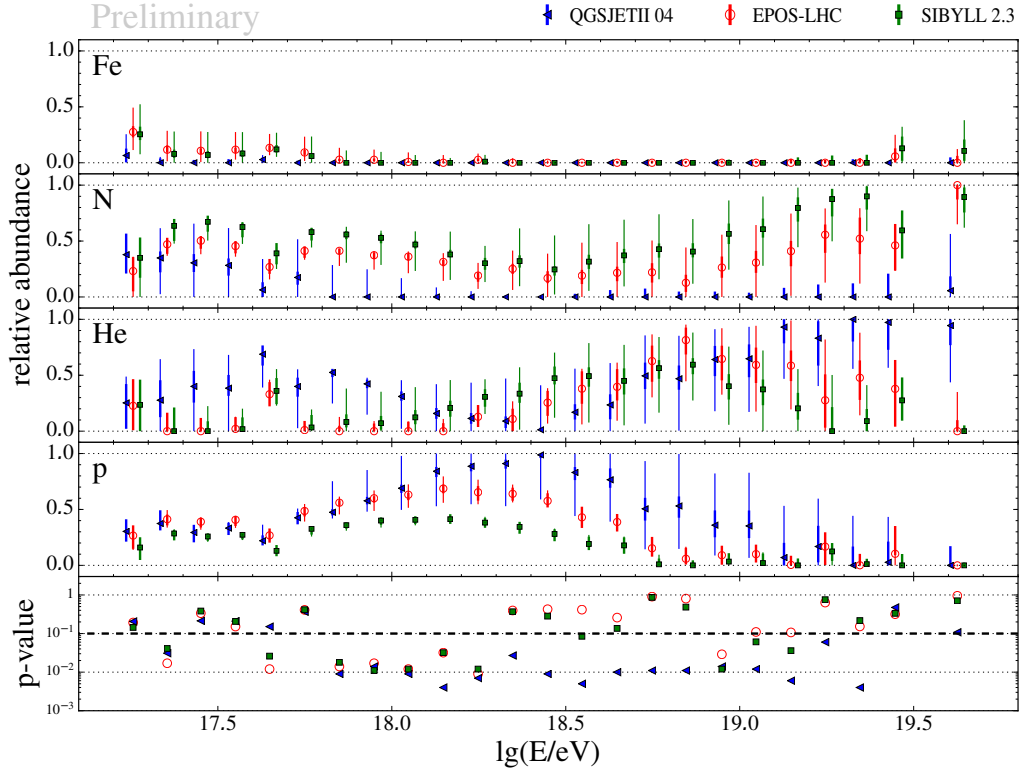
Figure 9. Relative abundance of four mass groups as function of energy in cosmic rays as measured by the Pierre Auger Observatory [165]. The upper four panels show the best-fit mass fractions and the goodness of fit is displayed in the lowest panel. Thick error bars denote the statistical uncertainties, thin error bars the systematic ones. 8
