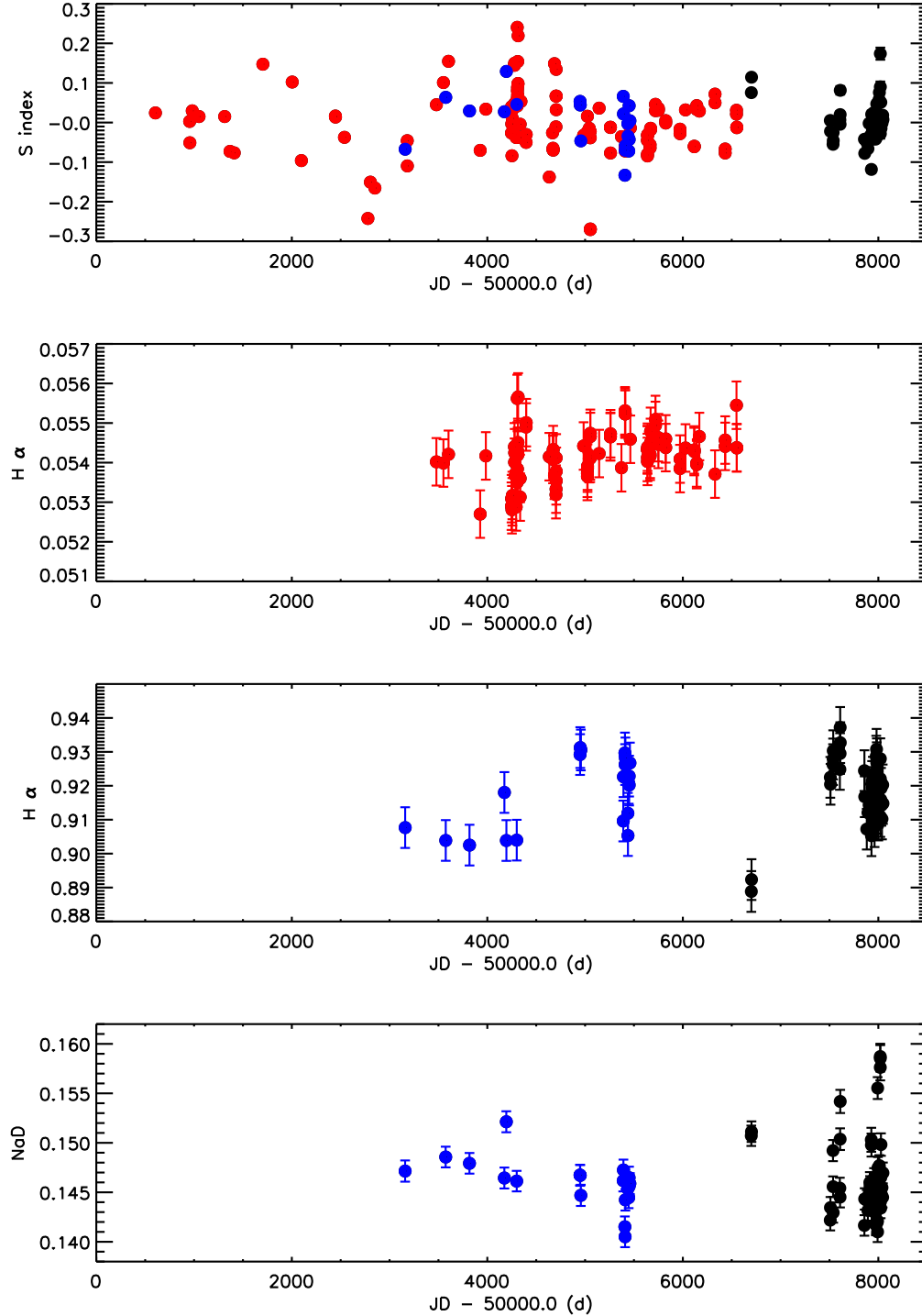
Fig. A.1. Time series data of the activity indexes, S -index (HIRES/red, HARPS/blue, HARPS-N/black), H\alpha (HIRES/red), H\alpha , and \text{NaD} (HARPS/blue, HARPS-N/black), from top to bottom panels.
