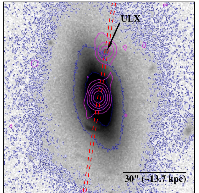
Figure 2. g-band image of NGC 5252 from the Sloan Digital Sky Survey. Blue contours represent the surface brightness. Magenta contours represent radio continuum at 20 cm from the FIRST survey. The ULX appears to have optical and radio counterparts. The long-slit position is denoted by the red dashed lines. North is up and east is left.
