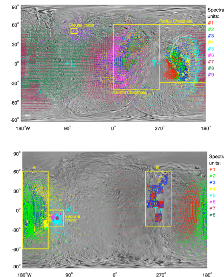
Figure 2: Homogeneous terrain units identified on Dione' (TOP) and Rhea' (BOTTOM) surface by applying the Spectral Angle Mapper classification technique to their VIMS spectra
