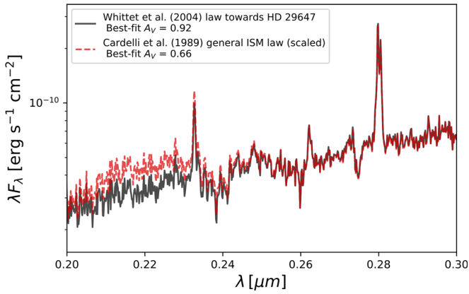
Figure 2. Spectra of CVSO 90 dereddened with the best-fit V-band extinction when modeled with the Whittet et al. (2004) law (black solid line) and Cardelli et al. (1989) law (red dashed line, shown scaled to the Whittet et al. 2004 law spectrum at 3000 Å). The overcorrected 2175 Å bump is apparent in the red curve.
