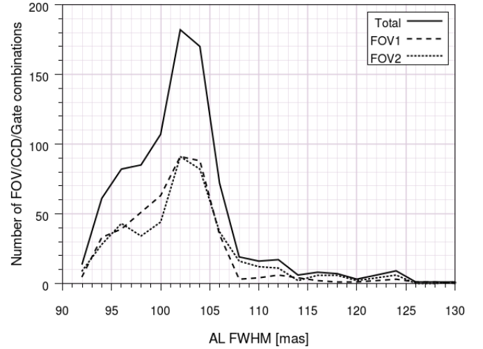
Fig. 6. Histogram of the FWHM in the AL direction for all CUs in AF at a mean colour. The solid black line shows the total; the dashed and dotted lines show the preceding and following FoV respectively. The median FWHM is 103 mas (1.75 pixels). Figure extracted from Fabricius et al. (2016).
