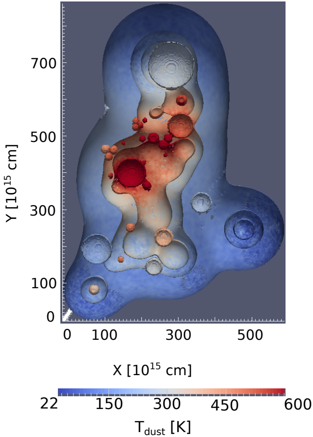
Fig. 7. Impression of the 3d view of the dust density distribution in Sgr B2(M). Three density isocontours are presented, i.e. at densities of 10^{-17.5} , 10^{-18} , and 10^{-19} g cm ^{-3} . They are colored using the dust temperature. The model is cut open at the model center to allow us a view inside. The bubbles are the empty half-shells of the distributed HII regions, which are free of dust. The dust on the surface of these HII regions is heated by the UV radiation field from the young stellar object embedded in the HII region. This dust is thus very hot, exceeding dust temperatures of 600 K (dark red spots). Visible here are mainly the HII regions detected by (De Pree et al. 1998, F1a – F4d).
