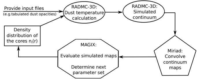
Fig. 2. Flowchart of the modeling framework pandora.
