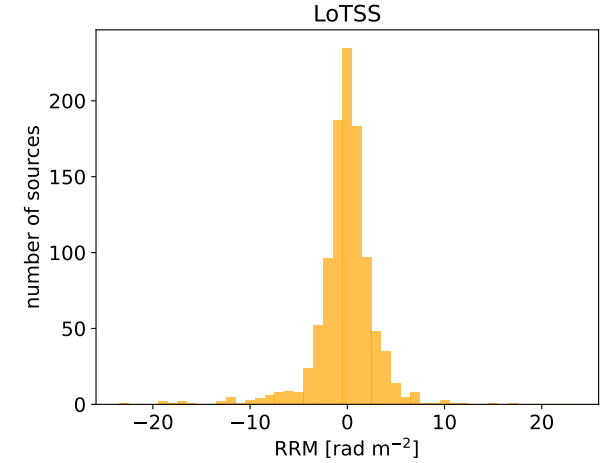
Figure 3. Distribution of RRM of the sample from the LoTSS RM catalogue
