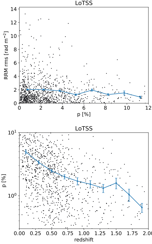
Figure 6. Top: RRM rms deviation as a function of fractional polarization p of the LoTSS sample (solid line). Individual |\text{RRM}| s are also reported (dots). Bottom: Mean of the fractional polarization p as a function of z of the LoTSS sample (solid line). Individual fractional polarizations are also reported (dots).
