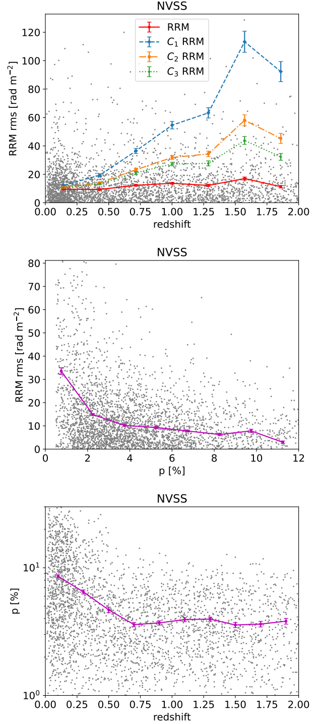
Figure 8. Top: NVSS sample RRM rms deviation in redshift bins (red solid line). The rest frame \text{RRM}_0 corrected for the redshift effect C_1 (dashed line), C_2 (dot-dashed line), and C_3 (dotted) are also plotted. The individual |\text{RRM}| s are reported as dots. Middle: RRM rms deviation as a function of fractional polarization p for the NVSS sample (solid line). Individual |\text{RRM}| values are also reported (dots). Bottom: Mean of fractional polarization p as a function of z for the NVSS sample (solid line). Individual fractional polarization values are also shown (dots).
