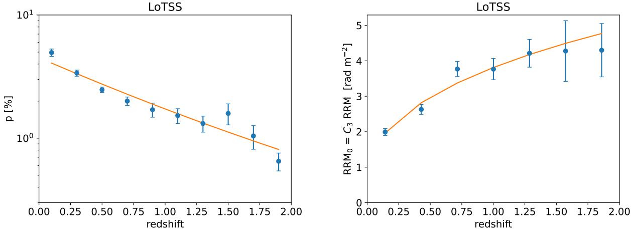
Figure 15. Left: Polarization fraction p versus redshift of the LoTSS sample (circles) and best fit of the function of Equation (21) (solid line). Right: \text{RRM}_0 as a function of redshift of the LoTSS sample corrected for model C_3 (circles) and best fit of the function of Equation (24) (solid line).
