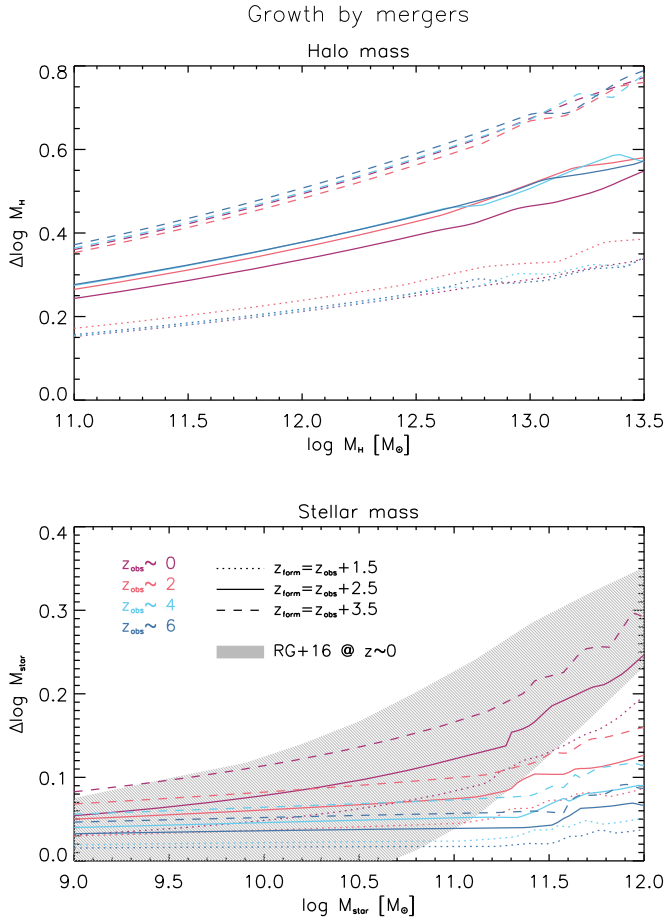
Figure 4. Growth of the halo mass (top panel) and stellar mass (bottom panel) by mergers as a function of the final halo and stellar masses, respectively. We illustrate the outcomes at observation redshifts z_{\text{obs}} = 0 (red), 2 (orange), 4 (cyan), and 6 (blue) for different formation redshifts z_{\text{form}} = z_{\text{obs}} + 1.5 (dotted), z_{\text{obs}} + 2.5 (solid), and z_{\text{obs}} + 3.5 (dashed). For z_{\text{obs}} = 0 , we also show the typical stellar mass growth via mergers from the Illustris simulation by Rodriguez-Gomez et al. (2016; gray shaded area).
