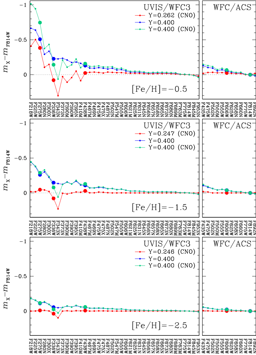
Figure 5. Colour difference between each isochrone of Fig. 3 and the black isochrone for UVIS/WFC3 (left) and WFC/ACS filters (right). The colour difference corresponding to the five X filters available for all the clusters of this paper, namely F275W, F336W, F438W, F606W, and F814W, are marked with large dots. Upper, middle, and lower panels correspond to [\text{Fe}/\text{H}] = -0.5 , -1.5 , and -2.5 , respectively. The colour differences have been calculated at the level of the dashed-dot lines plotted in Fig. 3, 2.0 F814W magnitudes above the MS turn off of the black isochrone.
