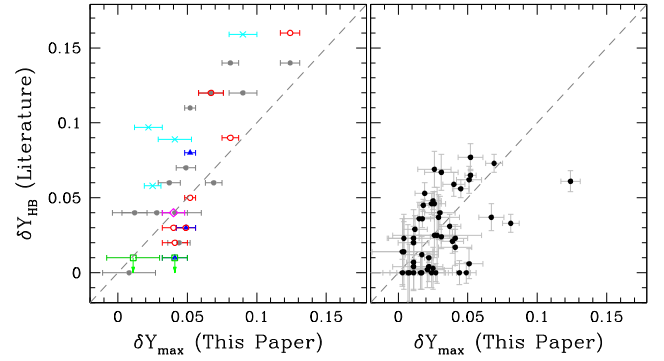
Figure 18. Comparison between the maximum helium abundance derived in this paper and the helium spread used in literature papers to reproduce the HB ( \delta Y_{\text{HB}} ). In the left-hand panel we show the values of \delta Y_{\text{HB}} adopted by D’Antona & Caloi (2008), Caloi & D’Antona (2007), and Tailo et al. (2017), which are represented as grey dots, while those from Busso et al. (2007), Dalessandro et al. (2011), Cassisi et al. (2014), and Salaris et al. (2016) are indicated by red circles. The helium spread used by Catelan et al. (2009) and Valcarce et al. (2016) are represented by green squares, while blue triangles and magenta diamonds indicate results by Denissenkov et al. (2017) and Campbell et al. (2013), respectively. Cyan crosses refer to the helium-difference estimates provided by Jang et al. (2014), Joo & Lee (2013), and Lee et al. (2009). In the right-hand panel we show the comparison with Gratton et al. (2010).
