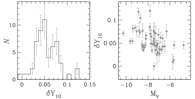
Figure 19. Left-hand panel: Histogram distribution of \delta Y_{1\text{G}} for the clusters studied in this paper. Right-hand panel: \delta Y_{1\text{G}} as a function of the absolute magnitude of the host GC.
