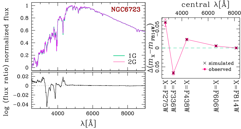
Figure 10. The aqua and magenta synthetic spectra plotted in the upper-left-hand panel correspond to 1G and 2G stars of NGC 6723 with m_{F814W} = 16.38 , respectively. Lower-left-hand panel shows the logarithm of the flux ratio of 2G and 1G spectra as a function of wavelength. Right-hand panel reproduces the plot of Fig. 9 where we show with magenta points the \Delta(m_X - m_{F814W}) colour difference between 2G and 1G fiducials of NGC 6723 with m_{F814W} = 16.38 against the central wavelength of the X filter. The black crosses overimposed on this plot are the corresponding colour difference derived from synthetic spectra.
