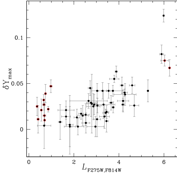
Figure 16. Maximum internal helium variation, \delta Y_{\max} , against the F275W–F814W colour extension of the HB. Metal-rich clusters with [\text{Fe}/\text{H}] > -0.99 are marked with red circles.
