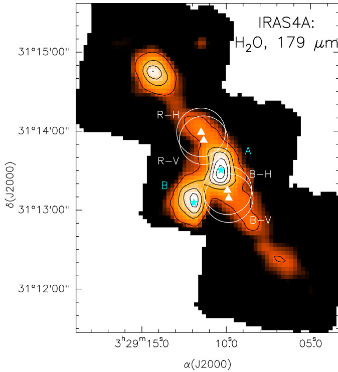
Figure 1. NGC 1333 IRAS4A outflow and corresponding observed positions. The background image represent the H_2O emission at 179 \mu m from the WISH program (Santangelo et al. 2014). The circles show the vertical (V) and horizontal (H) polarization HPBW at the observed positions, whose centers are indicated by the triangles. The stars mark the position of the continuum sources (A and B: Looney, Mundy & Welch 2000).
