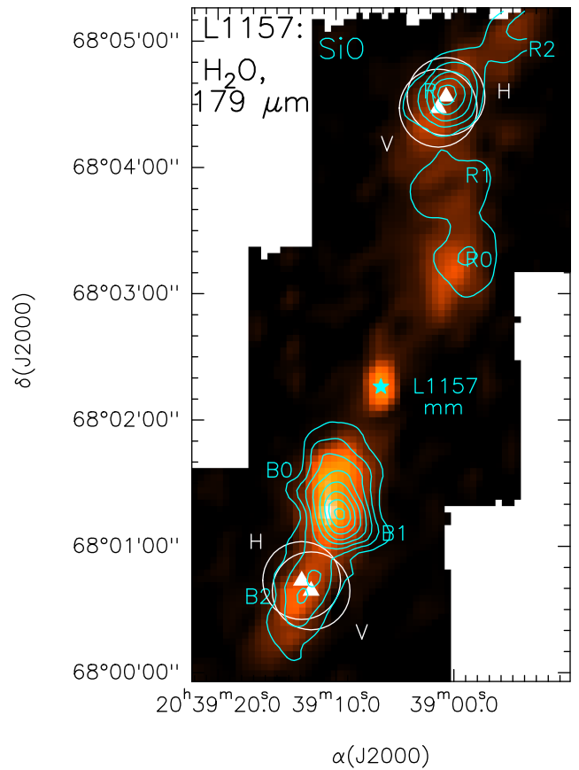
Figure 2. L1157 outflow and corresponding observed positions. The background image represent the H_2O emission at 179 \mu m from the WISH program (Nisini et al. 2010). The blue contours show the SiO emission from Bachiller et al. (2001). The circles show the vertical (V) and horizontal (H) polarization HPBW at the observed positions, whose centers are indicated by the triangles. The star marks the position of the central source (L1157-mm).
