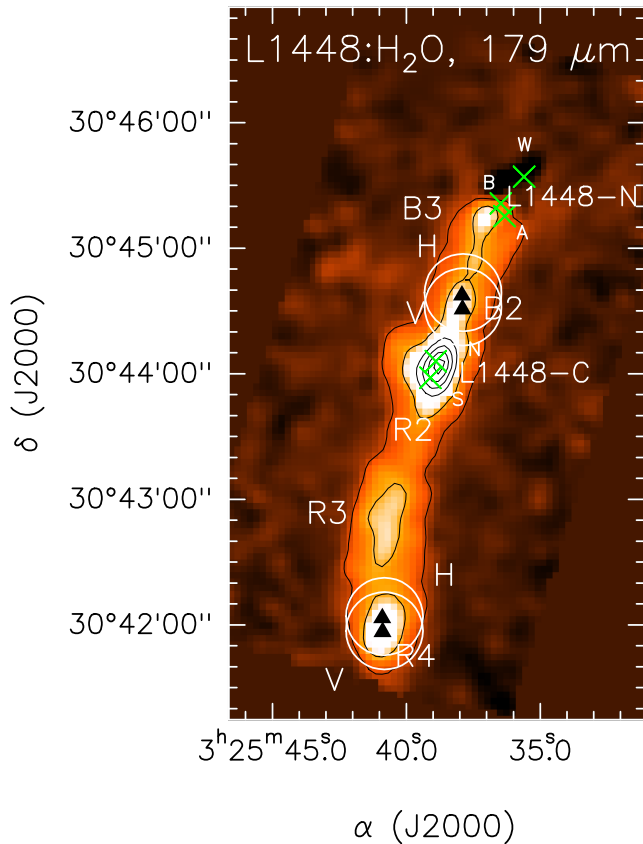
Figure 3. L1448 outflow and corresponding observed positions. The background image represent the \text{H}_2\text{O} emission at 179 \mu\text{m} from the WISH program (Nisini et al. 2013). The circles show the vertical (V) and horizontal (H) polarization HPBW at the observed positions, whose centers are indicated by the triangles. The green crosses indicate the positions of the millimeter continuum sources (N, S, A, B, and W: Kwon et al. 2006).
