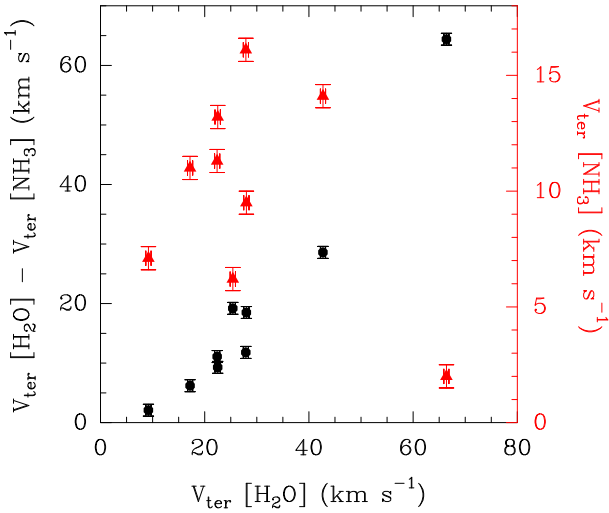
Figure 8. Comparison between the maximum (terminal, V_{\text{ter}} ) velocity (absolute values with respect to the systemic velocity, see Table 4) of the \text{H}_2\text{O} emission at 179 \mu\text{m} and that of \text{NH}_3 at 572 \text{ GHz} . Black points show the comparison between V_{\text{ter}}[\text{H}_2\text{O}] - V_{\text{ter}}[\text{NH}_3] versus V_{\text{ter}}[\text{H}_2\text{O}] , while red points compares V_{\text{ter}}[\text{NH}_3] with V_{\text{ter}}[\text{H}_2\text{O}] .
