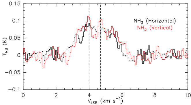
Figure 6. High spectral resolution (HRS) \text{NH}_3 spectrum towards L1448-B2. Horizontal and Vertical polarization are shown in black and red, respectively. The vertical dashed lines indicate the velocities of the two clouds ( 4.0 \text{ km s}^{-1} and 4.7 \text{ km s}^{-1} ) found in ammonia centimeter transitions by Bachiller & Cernicharo (1986).
