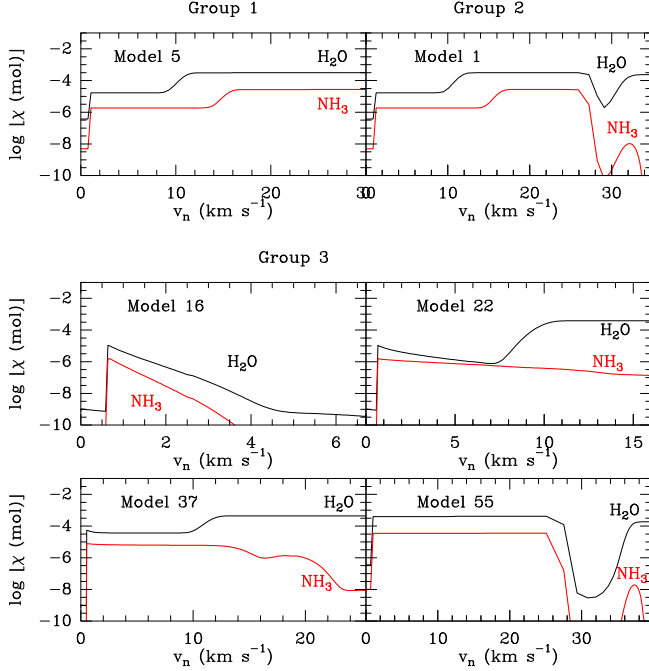
Figure 9. Fractional abundances with respect to the total number of hydrogen nuclei of water and ammonia as a function of velocity within the postshock gas, for representative models within each Group.
