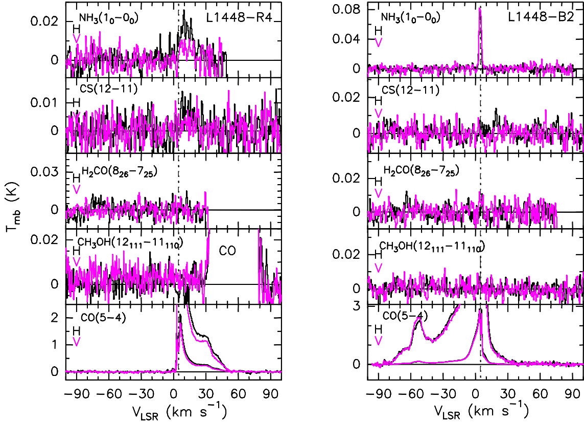
Figure A2. Same as Fig. A1 but for L1448 positions.
