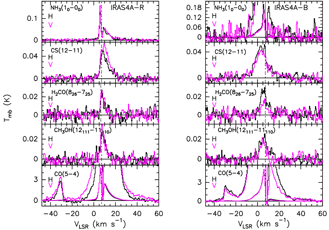
Figure A4. Same as Fig. A1 but for IRAS4a positions. Note that contamination from the image band of the \text{CH}_3\text{OH} 6(1, 6)-5(0, 5) transition ( E_u \sim 62 K, \nu_0 = 584.4499 GHz) is seen at V_{\text{LSR}} \sim -30 km s ^{-1} .
