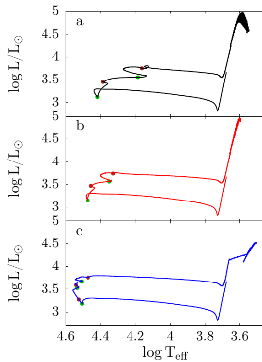
Figure 2. Hertzsprung–Russell diagrams of the three 6 M_{\odot} models with initial metallicity Z = 10^{-4} (panel a ), Z = 10^{-6} (panel b ) and Z = 10^{-10} (panel c ). The formation and the exhaustion of each convective core are marked with green and brown dots, respectively.
