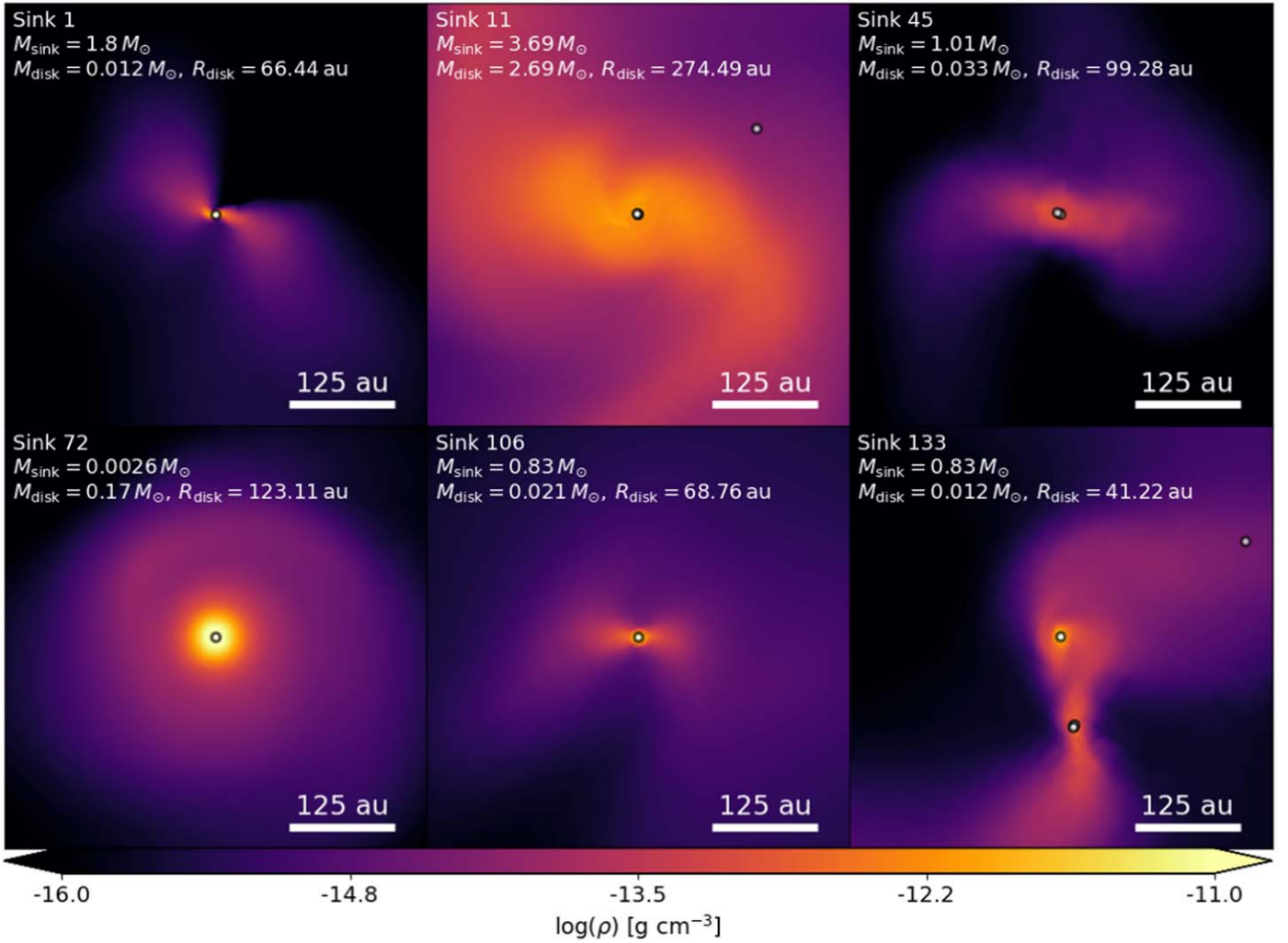
Figure 2. IMHD at t_{160M_{\odot}} = 118 \text{ kyr} . Same as the top six snapshots of Figure 1.
