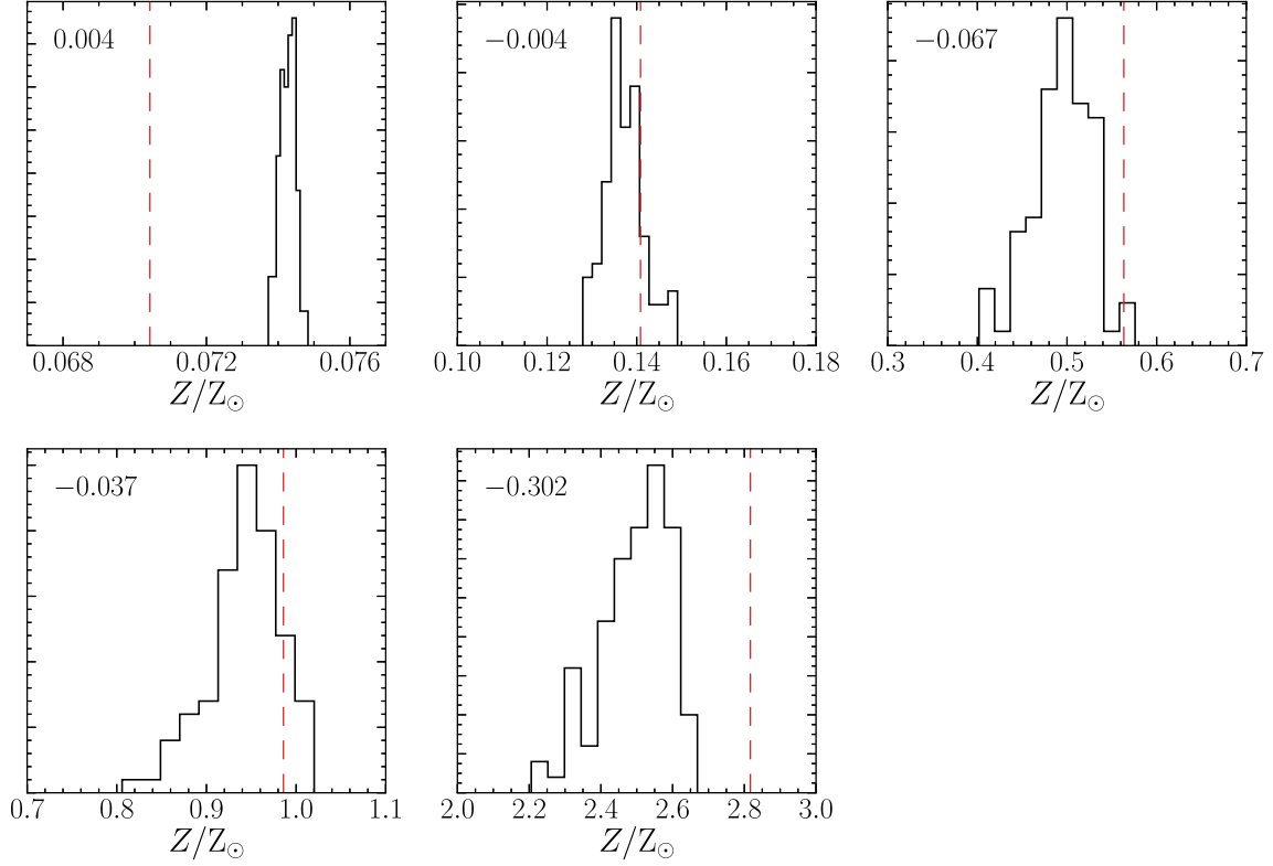
Figure B1. The distribution of recovered metallicity for each of the five default Starburst99 WM-Basic template spectra ( Z_* = 0.001, 0.002, 0.008, 0.014 , and 0.040 ) after mimicking the effect of redshift uncertainties when creating composite spectra (see text for details). Each panel shows one of the five default templates with the true metallicity indicated by the dashed vertical red line. The distribution of recovered metallicities is shown in black. The offset between the median recovered metallicity and the true metallicity is quoted in the top left-hand corner of each panel.
