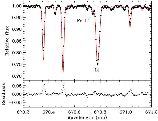
Fig. 7. Top panel: Lithium doublet of the solar analog KIC 10644253 observed with the HERMES instrument (dots) around 670.7 nm and associated spectral synthesis (red solid line) calculated using the spectroscopic set of atmospheric parameters given in Table 5. Bottom panel: residuals between the observed and the synthetic spectra.
