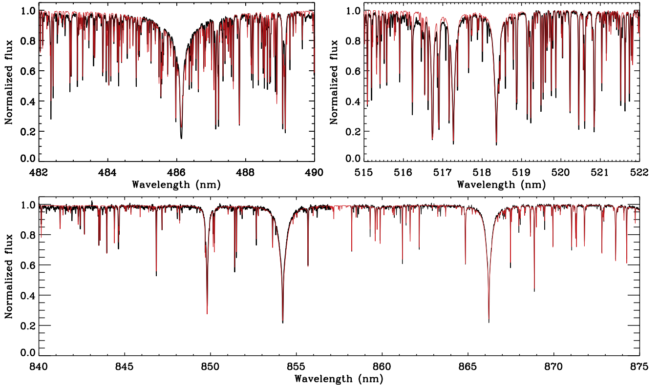
Fig. 5. Examples of the normalized spectrum of KIC 10644253 (in black) collected by the HERMES spectrograph over three different wavelength ranges, respectively around the lines H_\beta (top-left panel), Mg II (top-right panel), and the Ca IRT triplet (bottom panel). The associated best fitting synthetic spectra are represented in red.
