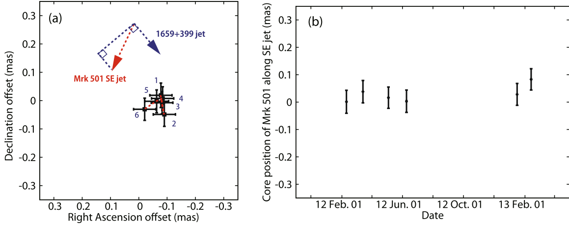
Figure 9. Measured radio core position of Mrk 501 relative to the radio core of calibrator 1659+399. (a) The blue arrow indicates the jet direction of 1659+399, and the red arrow indicates the direction of Mrk 501's SE jet. (b) The horizontal and vertical axes show the time and the positional offsets along the direction of Mrk 501's SE jet with respect to the position of the first epoch. The positional offsets are extracted along the perpendicular direction to the jet of 1659+399 and recalculated along the direction of Mrk 501's SE jet.
