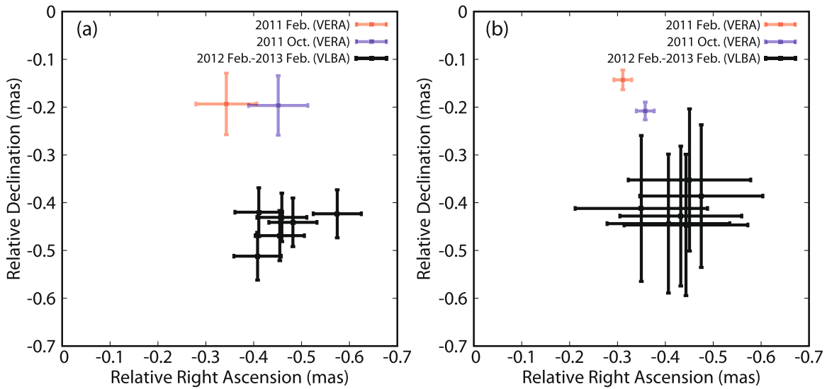
Figure 6. (a) Core positions of Mrk 501 relative to 3C 345's core. The positions measured with the VLBA are the same as those in Figure 2. (b) Core positions of NRAO 512 relative to 3C 345's core. The positions measured with the VLBA are obtained by subtracting the core positions in Figure 5 from those in Figure 6(a). The VLBA measurements are shown as black crosses, and the VERA measurements are shown as red and blue crosses, which are averaged over four successive measurements in 2011 February and October, taken from Figures 4(a) and (b), respectively, in Koyama et al. (2015).
