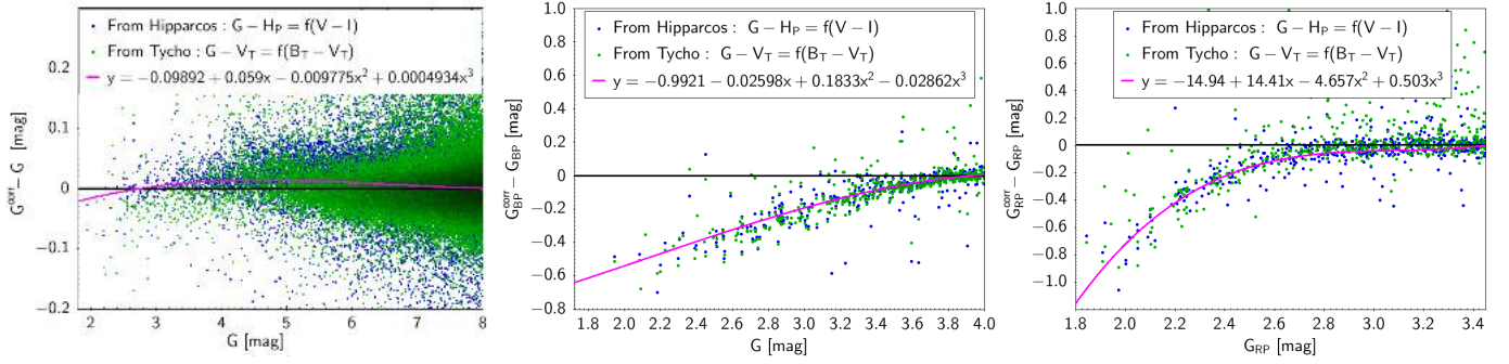
Fig. C.2. Saturation corrections for G (left), G_{\text{BP}} (centre) and G_{\text{RP}} (right) passbands.
