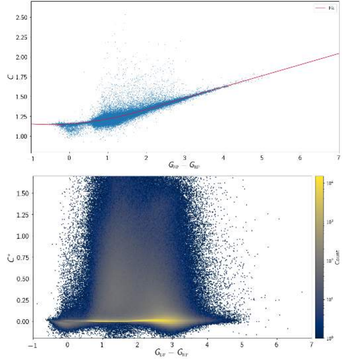
Fig. 18. Determination of the BP and RP flux excess dependence on G_{BP} - G_{RP} colour and its application to define the corrected excess factor C^* . Top panel: BP and RP flux excess vs. G_{BP} - G_{RP} colour for the set of standard sources from Stetson (2000) secondary standards and Ivezić et al. (2007). The red line represents the combined fit based on two different polynomials for the bluer-end and the central region and a linear fit for the red-end. Bottom panel: corrected flux excess factor C^* vs. G_{BP} - G_{RP} colour for a set of nearby sources selected from the Gaia EDR3 archive.
