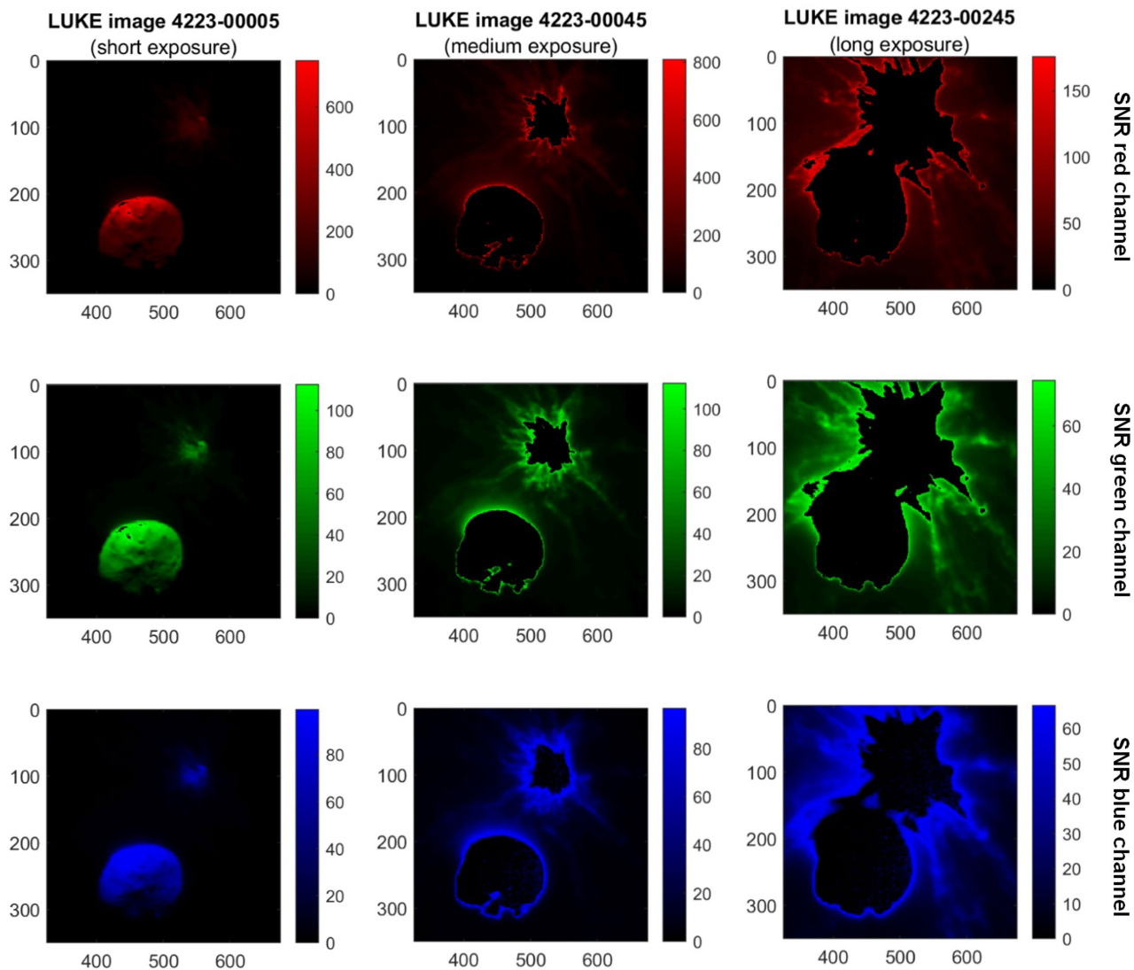
Extended Data Fig. 6 | Signal to Noise values for RGB channels in LUKE images. The showed S/N have been evaluated from background of images acquired at time 2022-09-26T23:17:03.000Z (0.5 ms exposure time, SCLK
