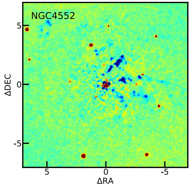
Figure 9. HST dust absorption map of NGC 4552. The dust absorption appears in blue in this color scale, zero emission is green, and the red areas represent residual emission or emission bluer than the average stellar population in the galaxy.
