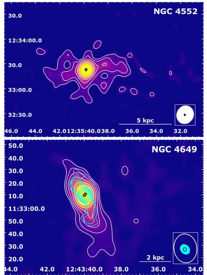
Figure 15. VLA radio total intensity maps at 1–2 GHz for NGC 4552 (top) and NGC 4649 (bottom) in the C and D configurations, respectively. The maps are overlaid by the white contours of these compact configurations; black is for the VLA A configuration, and cyan is for the VLA B configuration contours (previously published by Dunn et al. 2010). In all cases, the contours are created at [1, 2, 4, 8, 16, \dots] \times 5 rms noise and the restoring beams (resolution) are shown in the bottom-right corner of all radio maps (for more details, see Table 5).
