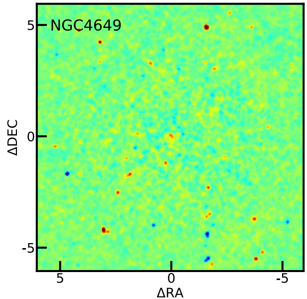
Figure 10. HST dust absorption map of NGC 4649. There is no evidence of dust in absorption in the central \sim 1.2 kpc.
