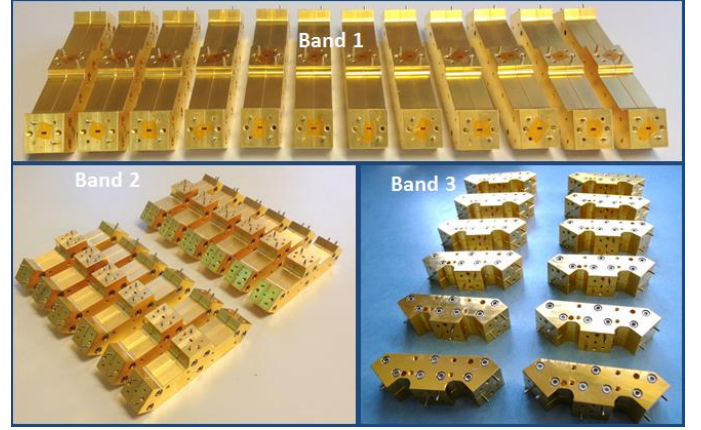
Fig. 15. Cryogenic LO splitters produced and characterized for NOEMA Bands 1, 2 and 3.
