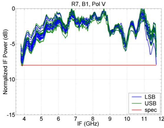
Fig. 27. Normalized IF output powers from LSB (blue curve) and USB (green curve) channels versus IF for 15 different LO settings (from 80 GHz to 108 GHz by steps of 2 GHz, 30 curves in total). The horizontal red line at -8 dB is the specification (8 dB peak-to-peak full band, see Tab. II).
