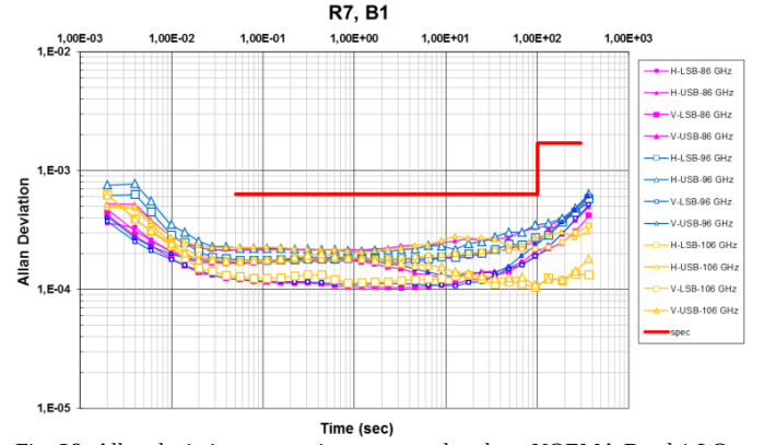
Fig. 29. Allan deviation versus time measured at three NOEMA Band 1 LO frequencies: 86 GHz (pink curves), 96 GHz (blue curves) and 106 GHz (yellow curves). For each LO setting, the four outputs (Pol. H-LSB, Pol H-USB, Pol V-LSB, Pol V-USB) are measured over the full IF bandwidth (~3.8-11.7 GHz).
