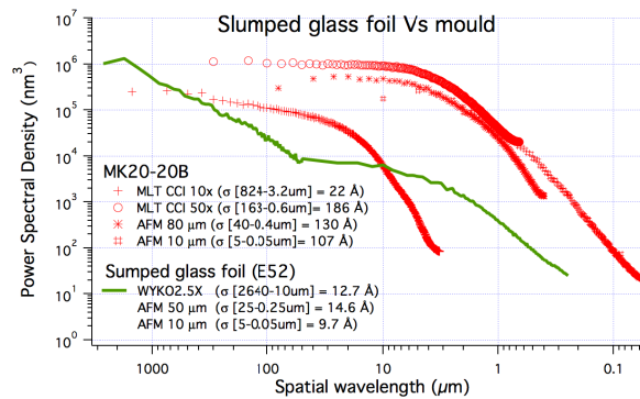
Fig. 4. PSD from roughness data obtained for the MK20-20B slumping mould (red line) and one Eagle glass foil slumped on it (green line, glass code E52).
