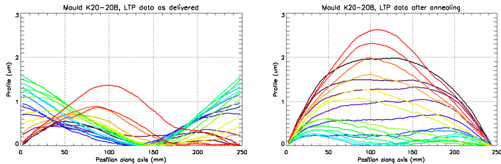
Fig. 13. LTP profiles of the MK20-20B, taken with steps of 1 mm in the longitudinal direction and every cm in the azimuthal direction. Left graph shows the as delivered mould: PV_{\text{center}} = 1.4 \mu\text{m} concave, PV_{90\text{mm-left}} = 0.6 \mu\text{m} concave, PV_{90\text{mm-right}} = 0.9 \mu\text{m} convex. Right graph shows the mould after the annealing for comparison: PV_{\text{center}} = 0.3 \mu\text{m} concave, PV_{90\text{mm-left}} = 2.1 \mu\text{m} convex, PV_{90\text{mm-right}} = 2.5 \mu\text{m} convex.
