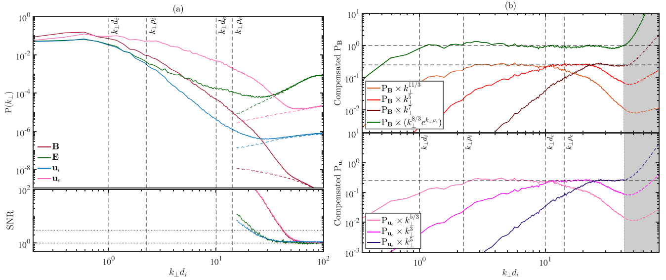
Figure 3. Spectral behavior of the electromagnetic and plasma fluctuations. (a) Power spectra of the magnetic field B , the electric field E , the ion bulk velocity u_i , and the electron bulk velocity u_e with the respective noise in dashed lines (top) and corresponding signal-to-noise ratio S/N (bottom). Vertical dashed black lines mark the particle characteristic scales, i.e., the ion and electron inertial length d_{i,e} and gyroradius \rho_{i,e} . (b) Power spectra of the magnetic field B (top) and of the electron bulk velocity fluctuations u_e (bottom), compensated by different power laws (and by an exponential cutoff for B ). The gray area marks the scales at which S/N < 3.
