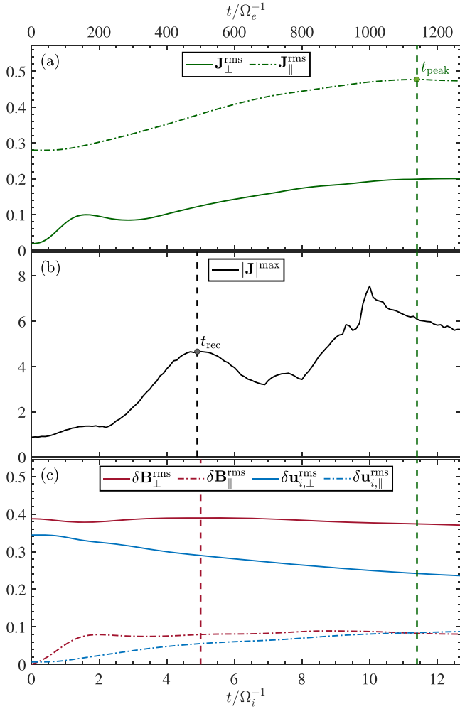
Figure 1. Time evolution of some global quantities. (a) The rms value of the out-of-plane and in-plane components of the current density, \mathbf{J}_{\perp} and \mathbf{J}_{\parallel} . (b) Maximum of the magnitude of the current density, |\mathbf{J}| , in the whole simulation box. (c) The rms of the components of the magnetic fluctuations, \mathbf{B}_{\perp} and \mathbf{B}_{\parallel} , and of ion bulk velocity, \mathbf{u}_{i,\perp} and \mathbf{u}_{i,\parallel} . In all panels, a vertical dashed green line marks the time when the rms of \mathbf{J}_{\parallel} reaches a maximum, i.e., when turbulence has fully developed. In panel (b), a vertical dashed black line marks the time when reconnection events start occurring, which also corresponds to the time when \mathbf{B}_{\perp} starts decreasing, indicated by the vertical dashed red line in panel (c).
