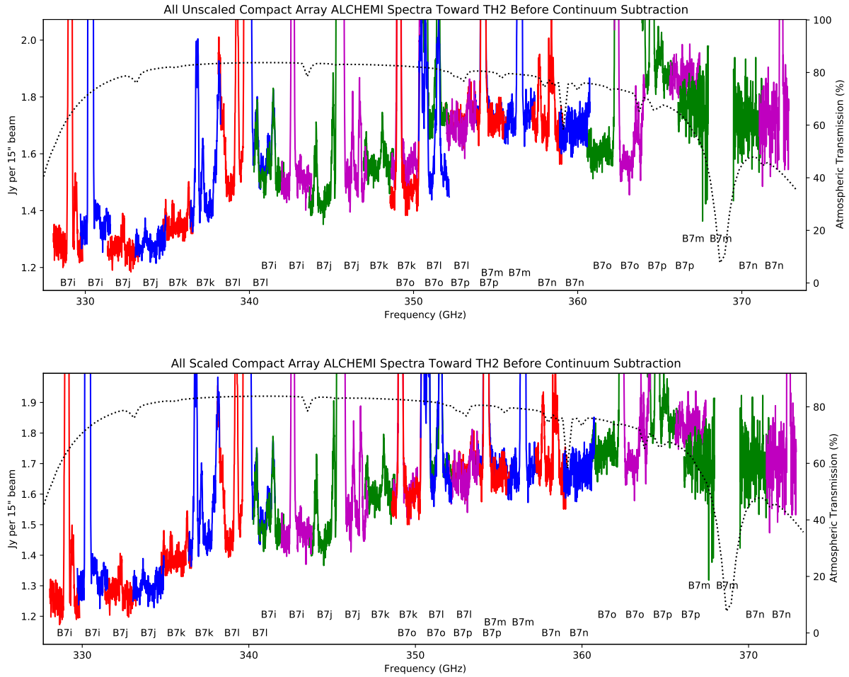
Fig. A.7. Same as Fig. A.2 but for the second half of Band 7 unscaled (top) and scaled (bottom).
