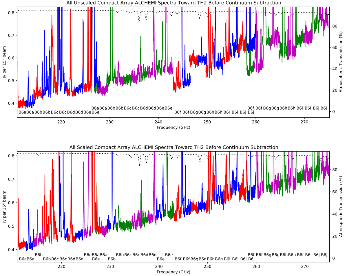
Fig. A.5. Same as Fig. A.2 but for Band 6 unscaled (top) and scaled (bottom).
