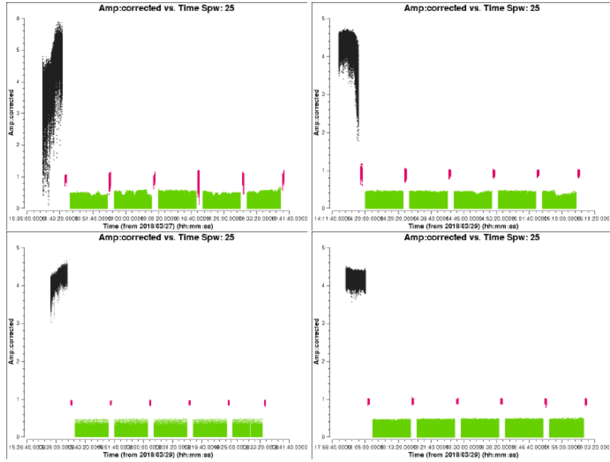
Fig. B.2. B3b 7m amplitude/bandpass calibrator flux versus time weblog plots for the four EBs in this SB.
