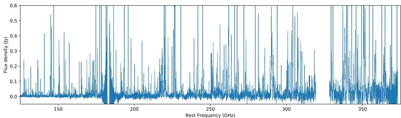
Fig. 4. Full spectral coverage obtained with the ALMA Compact Array (ACA 7m) alone, extracted from the position of brightest molecular emission (see Section 4.2.1). Fig. E.1 in Appendix E presents a zoomed version of this plot in 5 frequency windows 50 GHz wide where the comparison with the modeled emission (Sect. 4.2.2) and the molecular line identification of each individual feature is included. Figs. E.2–E.11 present a further zoomed version in 5 GHz windows.
