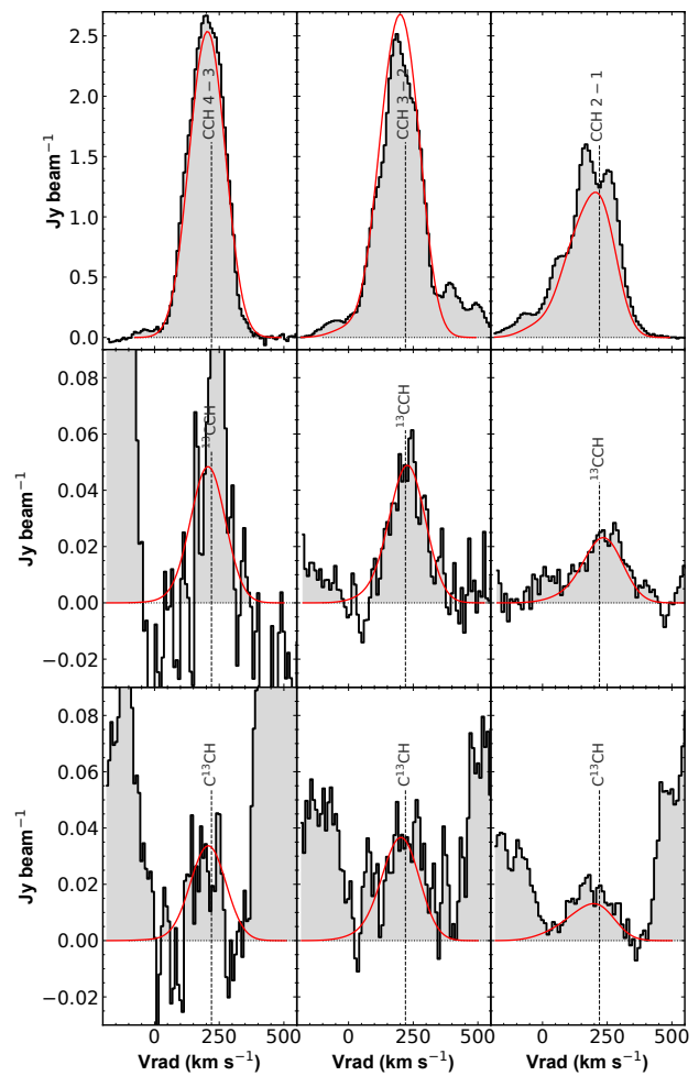
Fig. 14. Spectral features of the J = 4-3 (left), 3-2 (center) and 2-1 (right) transitions from three of the isotopologues of CCH detected in the survey. Red curves shows the LTE model best fits. Contributions by other species is almost negligible for most transitions according to the global LTE model from the full survey (see Sect. 4.2.2). However we note that the observed profile of ^{13}\text{CCH } 4-3 , not following the CCH LTE model and not accounted for by emission from other species, was not used in the fit.
