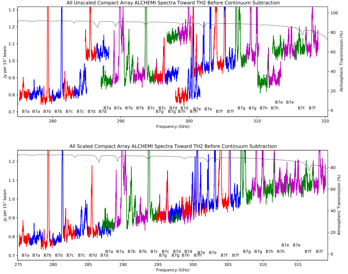
Fig. A.6. Same as Fig. A.2 but for the first-half of Band 7 unscaled (top) and scaled (bottom).
