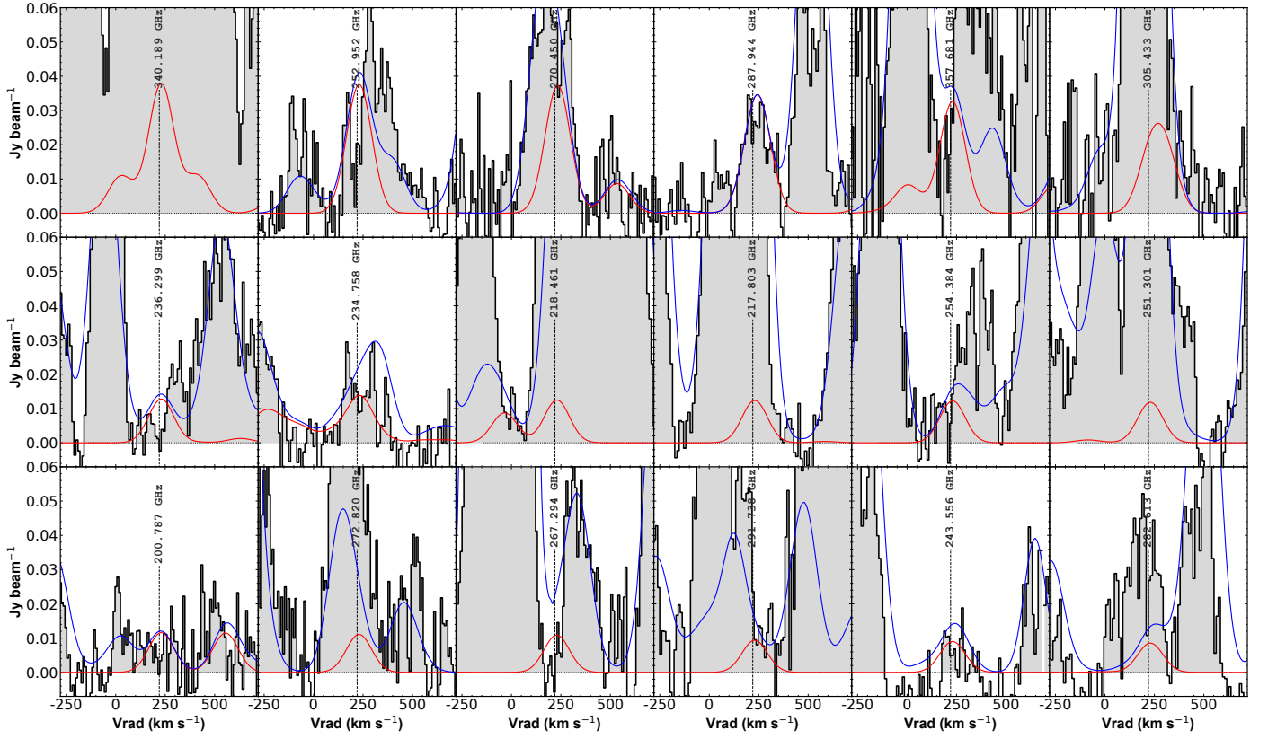
Fig. C.1. Modelled emission of \text{C}_2\text{H}_5\text{OH} in red, overlaid over the observed spectrum (filled black histogram) and the global model including all molecular transitions in this study. Only the 18 brightest transitions or group of transitions according to the LTE model of \text{C}_2\text{H}_5\text{OH} are displayed, ordered in descending order of brightness from left to right and top to bottom. The model generated with MADCUBA makes use of the spectroscopic parameters in JPL catalog entry 46004. The frequency of the brightest transition in each panel are displayed for reference.
