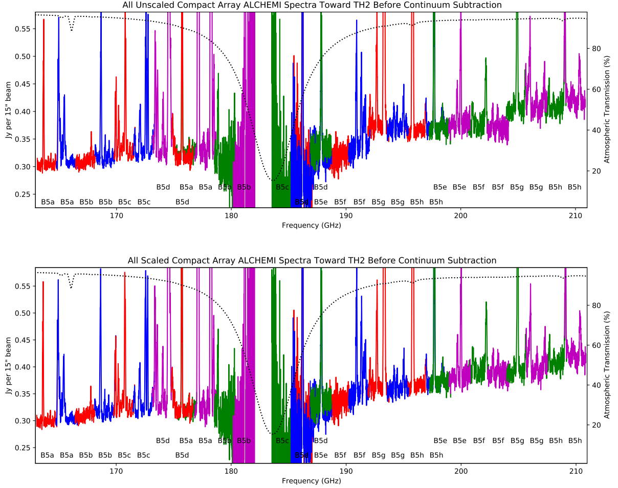
Fig. A.4. Same as Fig. A.2 but for Band 5 unscaled (top) and scaled (bottom).
