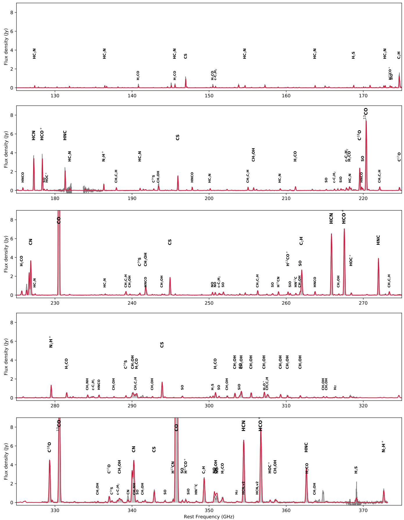
Fig. E.1. Full spectral coverage as in Fig.4 zoomed to 50 GHz frequency windows. The observed spectrum is shown in grey histogram and the model (Sect. 4.2.2) in red line. Only the brighter individual molecular transitions with intensities higher than 100 mJy are labeled with different y-axis position and character size depending on the modelled intensity for > 5 , > 1 , > 0.2 , and > 0.1 Jy.
