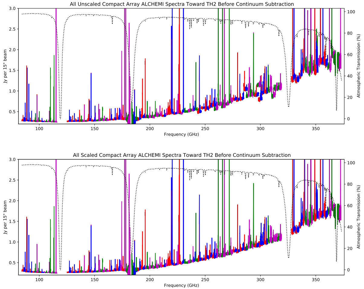
Fig. A.1. Unscaled (top) and scaled (bottom) full spectral scans. The spectra were extracted from the TH2 position in the low resolution data (see Sect. A). The colors in the spectra represent the spectral windows from the lower side band (red and blue) and the upper side band (green and violet). A dotted line indicates the atmospheric transmission for a PWV of 1 mm.
