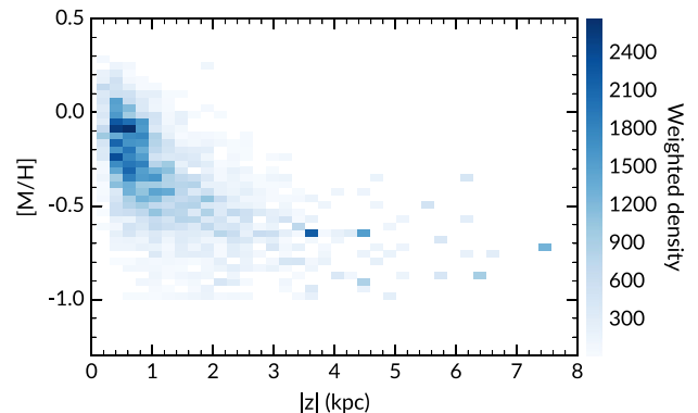
Figure 12. Variation of metallicity with distance from the Galactic plane for all stars independently of their \alpha assignment (the ‘transition’ stars mentioned in Section 3.3 are also included). The density was weighted using bias correction fractions described in Section 4. The metallicity decreases smoothly with increasing height; however, the gradient appears to flatten at |z| = 2 kpc.
