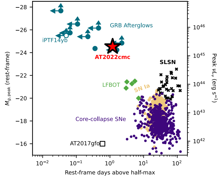
Extended Data Figure 2: Duration and luminosity of optical transients compared to AT2022cmc, including superluminous SNe (SLSN), Type Ia SNe (SN Ia), core-collapse SNe [66-68] , luminous fast blue optical transients (LFBOTs) [41, 42, 45-47, 68, 69] , GRB afterglows [69, 70] , and the kilonova AT 2017gfo [39, 71-74] .
