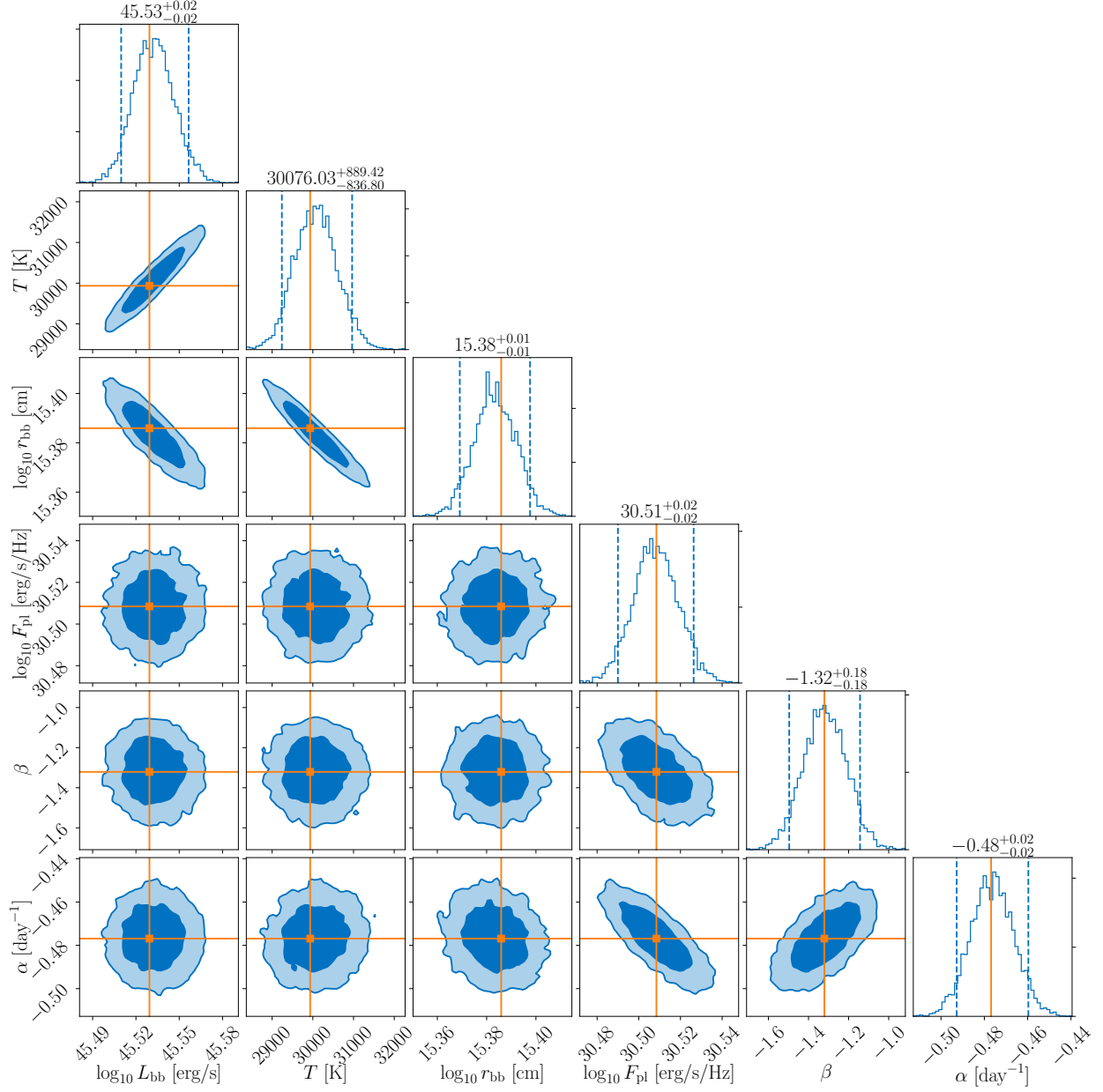
Extended Data Figure 4: Marginalized histograms for the optical light curve modelling discussed in Section 10 . The parameter estimates given correspond to median and 90% Bayesian credible intervals, as marked by the blue dashed vertical and horizontal lines. The best-fit (maximum likelihood) parameters are marked with the orange lines. The 68% (95%) credible regions are colored in dark (light) blue.
