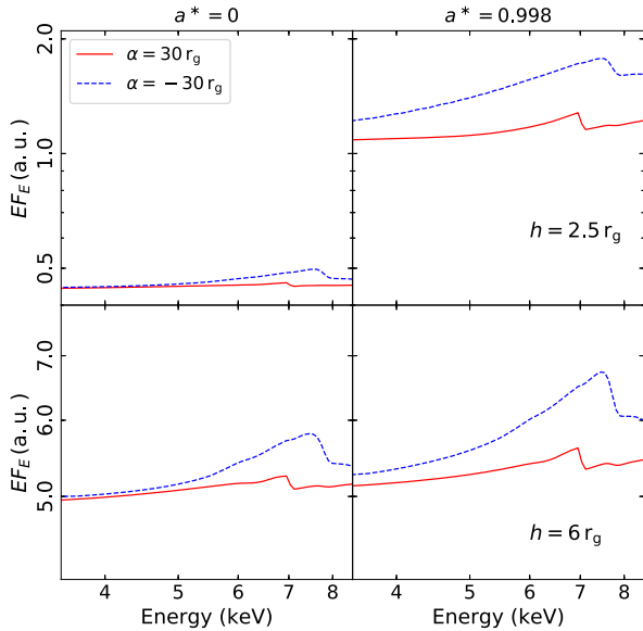
Figure 3. The observed spectra, in the 3.5\text{--}8.5\text{keV} range, considering a cloud of radius 30 r_g obscuring the approaching ( \alpha = 30 r_g , solid red lines) and receding ( \alpha = -30 r_g , dashed blue lines) parts of the accretion disc for BH spins of 0 (left-hand panels) and 0.998 (right-hand panels). We consider primary sources located at 2.5 and 6 r_g (top and bottom panels, respectively) above an accretion disc with an inclination of 60^\circ .
