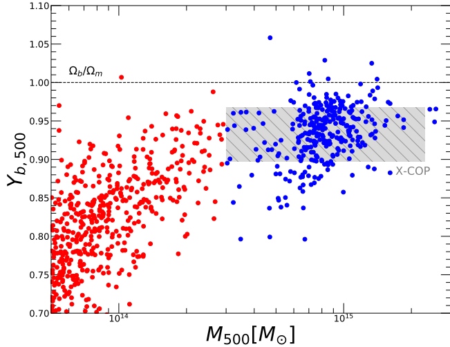
Fig. 2. Baryon depletion factor Y_b at R_{500} for the clusters in The300 simulation (filled circles). The blue points show the objects with a mass M_{500} > 3 \times 10^{14} M_\odot . The hashed gray shaded area shows the mass range covered by X-COP clusters and our determination of the universal baryon depletion factor and its scatter.
