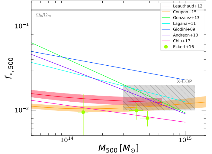
Fig. 3. Stellar fraction within R_{500} estimated in several works from the literature. The hashed grey area represents the mass range of X-COP clusters and the range of f_* adopted in this work.
