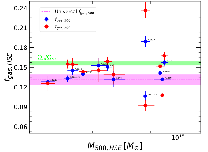
Fig. 4. Hydrostatic gas fractions at R_{500,\text{HSE}} (blue points) and R_{200,\text{HSE}} (red points) obtained from our reference hydrostatic mass model as a function of cluster mass. The dashed magenta line and shaded area represent the universal gas fraction at R_{500} estimated in Sect. 3.1 and its uncertainty. The green shaded area indicates the cosmic baryon fraction (Planck Collaboration XIII 2016).
