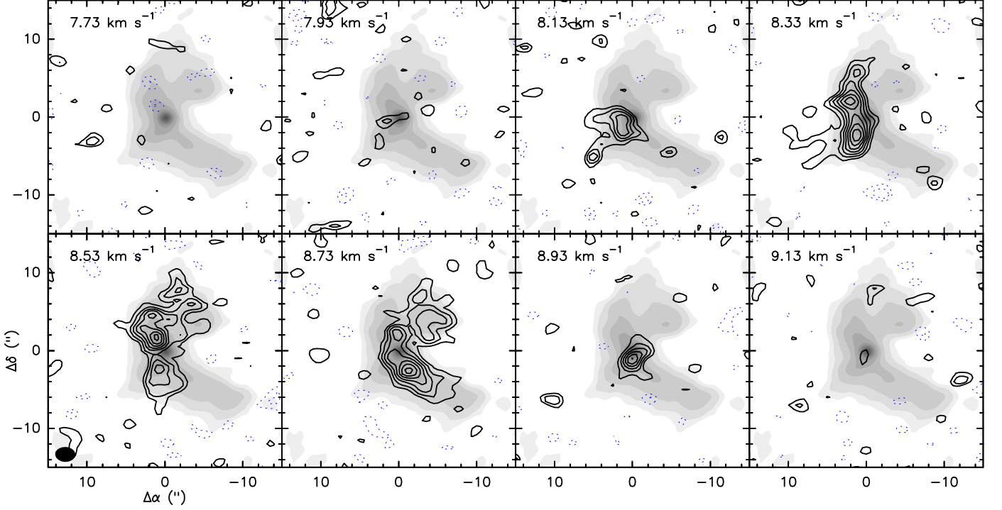
Fig. 3: Contour channel maps of the emission of the F=5/2-(-5/2) hyperfine component of the C^{17}O J=1-0 transition, overlapped with the gray scale image of the 1.3 mm dust emission. Contours are -4 , -2 , and from 2 to 18 by steps of 2 times the rms noise of the channel maps, 10 \text{ mJy Beam}^{-1} . The synthesized beam is shown in the bottom left panel as a filled ellipse. The v_{\text{LSR}} channel velocities are shown in the top left part of the panels.
