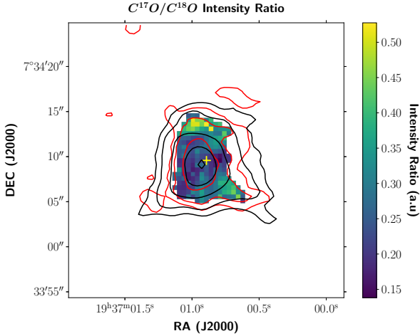
Fig. 4: C^{17}O to C^{18}O integrated intensity ratio. Red contours show integrated intensity for C^{17}O at -3 , 3 , 5 , 10 and 30 \sigma , where \sigma is 10.0 \text{ mJy/beam} . Black contours show integrated intensity for C^{18}O at -3 , 3 , 5 , 10 and 30 \sigma , where \sigma is 10.7 \text{ mJy/beam} . The yellow cross indicates the centroid position of B335.
