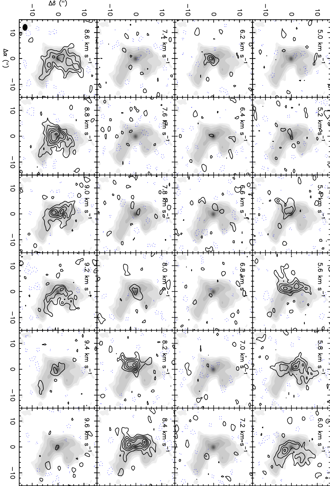
Fig. B.1: Contour channel maps of the \text{C}^{17}\text{O} (1-0) emission showing the two main hyperfine components, overlapped with the gray scale image of the 1.3 mm dust emission. Contours are -4 , -2 , and from 2 to 18 by steps of 2 times the rms noise of the channel maps, 10 \text{ mJy Beam}^{-1} . The synthesized beam is shown in the bottom left panel as a filled ellipse. The v_{\text{LSR}} channel velocities are shown in the top left part of the panels.
