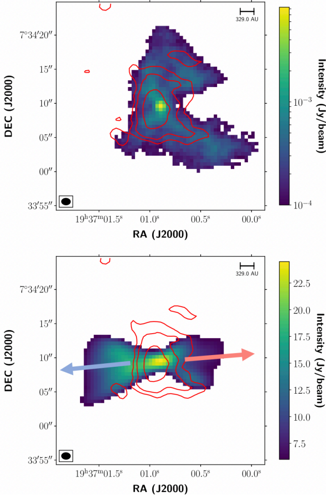
Fig. 1: Red contours showing moment 0 of C^{17}O emission, integrated over the velocity range 4.8\text{--}6.2\text{ km s}^{-1} and 7.6\text{--}9.4\text{ km s}^{-1} . Contours show emission at -3, 3, 5, 10 and 30\sigma , where \sigma is 10.0\text{ mJy/beam} . Top: Intensity shows dust continuum emission map at 110\text{ GHz} for emission over 3\sigma , where \sigma is 8.56 \times 10^{-2}\text{ mJy/beam} . Bottom: Intensity shows ^{12}CO (2-1) moment 0 emission integrated over the velocity range 1.4\text{--}16.2\text{ km s}^{-1} , for emission over 3\sigma , where \sigma is 2016.9\text{ mJy/beam} . The two arrows show the direction of the E-W outflow.
