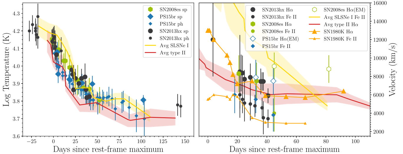
Figure 9. Left: SN2013hx (black) and PS15br (blue) temperature evolution compared with that of SN2008es (green). The gold region represents the 99.73 per cent region of the temperature space of SLSNe I (Inserra et al. 2013b; Nicholl et al. 2015), while the red denotes a Type II collection (Elmhadi et al. 2003; Maguire et al. 2010; Inserra et al. 2011, 2012a; Botticella et al. 2010; Tomasella et al. 2013; Gutiérrez et al. 2017b). Right: H \alpha and Fe II evolution of SN2013hx (black) and PS15br (blue) compared with that of SN2008es (green), the Type II SN1980K (orange triangle and line for H \alpha and smaller symbols for Fe II; Barbon et al. 1982). The gold region represents the velocity space of Fe II line in SLSNe I, while the red is that of H \alpha in SNe II. Open symbols refer to velocities computed with the FWHM of the emission lines.
