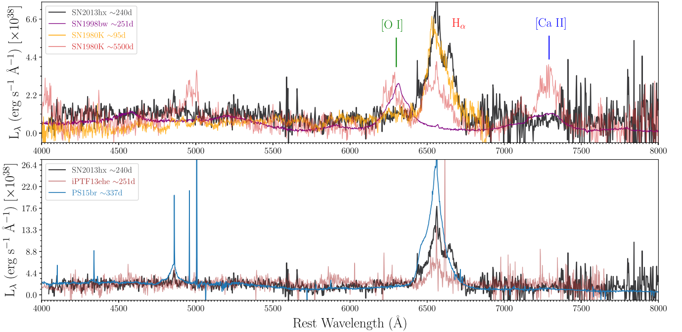
Figure 11. Top: the VLT+FORST2 spectrum of SN2013hx compared with late spectra of the SNe IIL SN1980K (Barbon et al. 1982) and a late spectrum of the broad-line SN Ic SN1998bw (Patat et al. 2001). All the spectra have been scaled to the continuum flux level of SN2013hx. The most prominent lines of nebular core-collapse spectra are labelled. Bottom: the VLT+FORST2 spectrum of SN2013hx and the VLT+XShooter (337d) compared with SLSNe I iPTF13ehe, a slow SLSN I showing late H\alpha emission.
