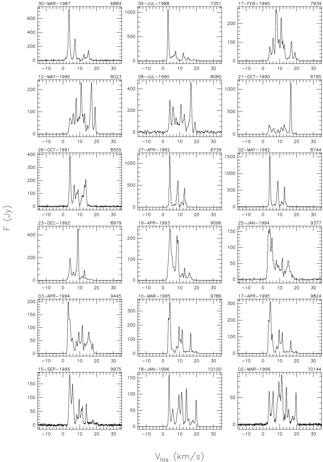
Fig. A.1. All H 2 O maser spectra of R Crt. The observing date ( top left ) and TJD ( top right ) are indicated for each spectrum.
