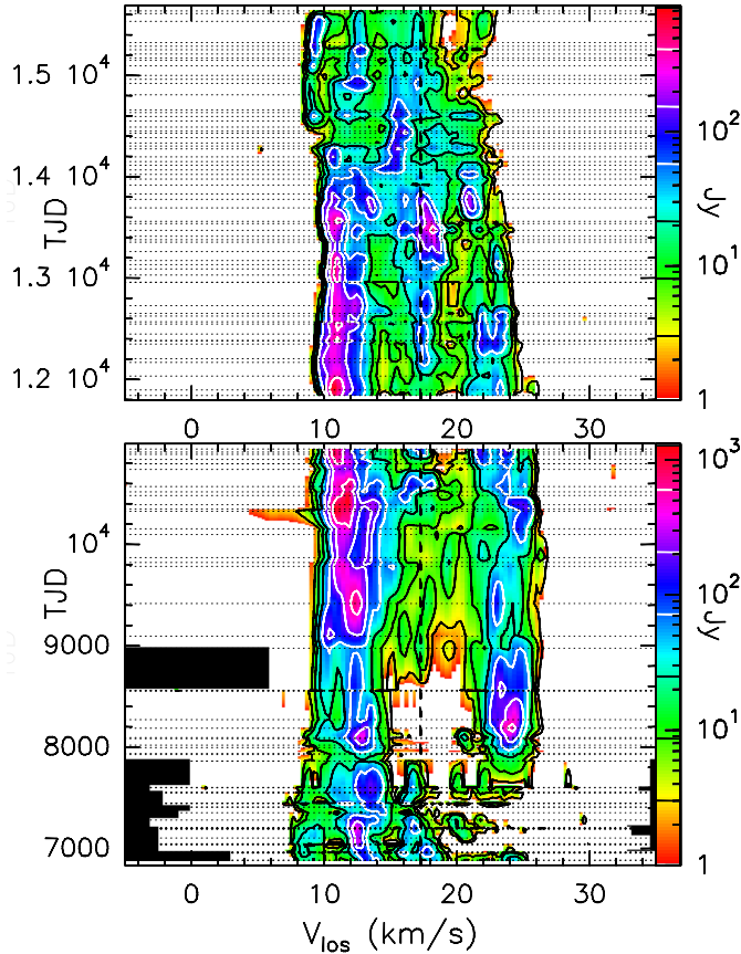
Fig. 8. As in Fig. 2, but for RT Vir. Lower panel: first spectrum: 1/4/1987; JD=2446886.5, TJD=6886 and last spectrum 11/5/1998. Upper panel: first spectrum 27/10/2000 and last spectrum 20/3/2011. The black areas in the plot indicate the unobserved parts of the spectrum on those particular days. The low-level emission at V_{\text{los}} \sim 4\text{--}10 \text{ km s}^{-1} at TJD = 10329 is an artefact.
