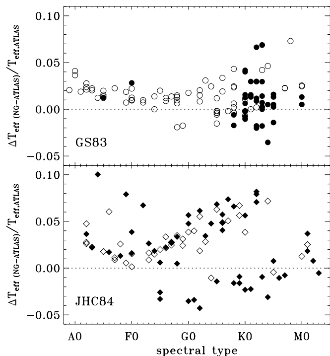
FIG. 12.—Temperature residuals for the 216 GS83 ( top ) and JHC84 stars ( bottom ) with both ATLAS and NextGen best-fit solution. Stars are labeled according to their MK luminosity class (MK IV–V, open markers ; MK I–III, filled markers ). Note, in the JHC84 plot, the peculiar distribution of giant stars along two distinct point sequences. Over the whole sample, NextGen tends to predict, on average, an effective temperature about 2% warmer than the ATLAS value (see text for a full discussion of these two important features).
