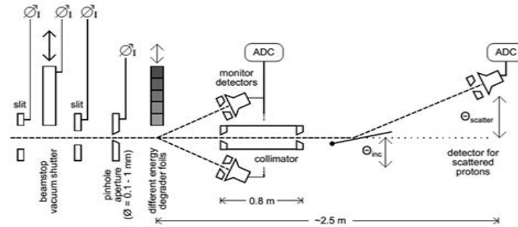
Figure 6. Schematic of the proton scattering setup implemented at the Van de Graaf accelerator of the University of Tuebingen.
