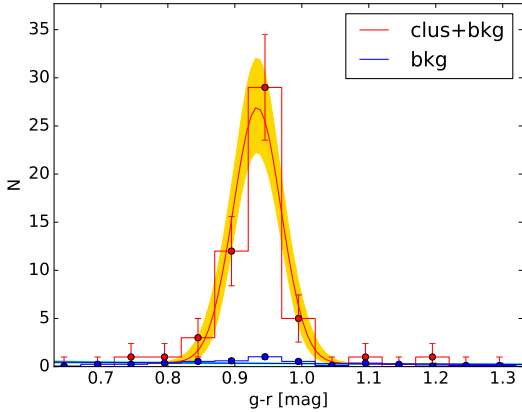
Figure 5. Illustration of red sequence width computing procedure for the cluster CL1001 as an example. The Gaussian+background fit (red curve), performed on unbinned counts, is overplotted to the binned red histogram/dots representing the cluster+background colour distribution; blue histogram/dots represent the binned background contribution superposed to the unbinned background fit (blue line). The yellow/cyan shadow indicates the 68% error.
