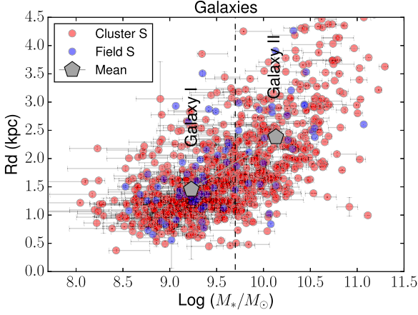
Figure 1. Replaces the right panel of Fig. 1 in the original paper (almost identical). The stellar mass ( M_* ) versus stellar disk scale length ( R_d ) of all the cluster and field spirals (S) from the WINGS/OmegaWINGS samples with a redshift. The pentagons indicate the properties of the model galaxies I and II.
