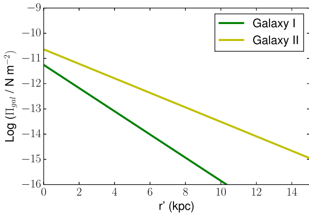
Figure 3. Replaces Fig. 4 in the original paper (both lines shifted). The anchoring force as a function of radial distance from the galaxy centre for two model galaxies (I and II, as indicated).
