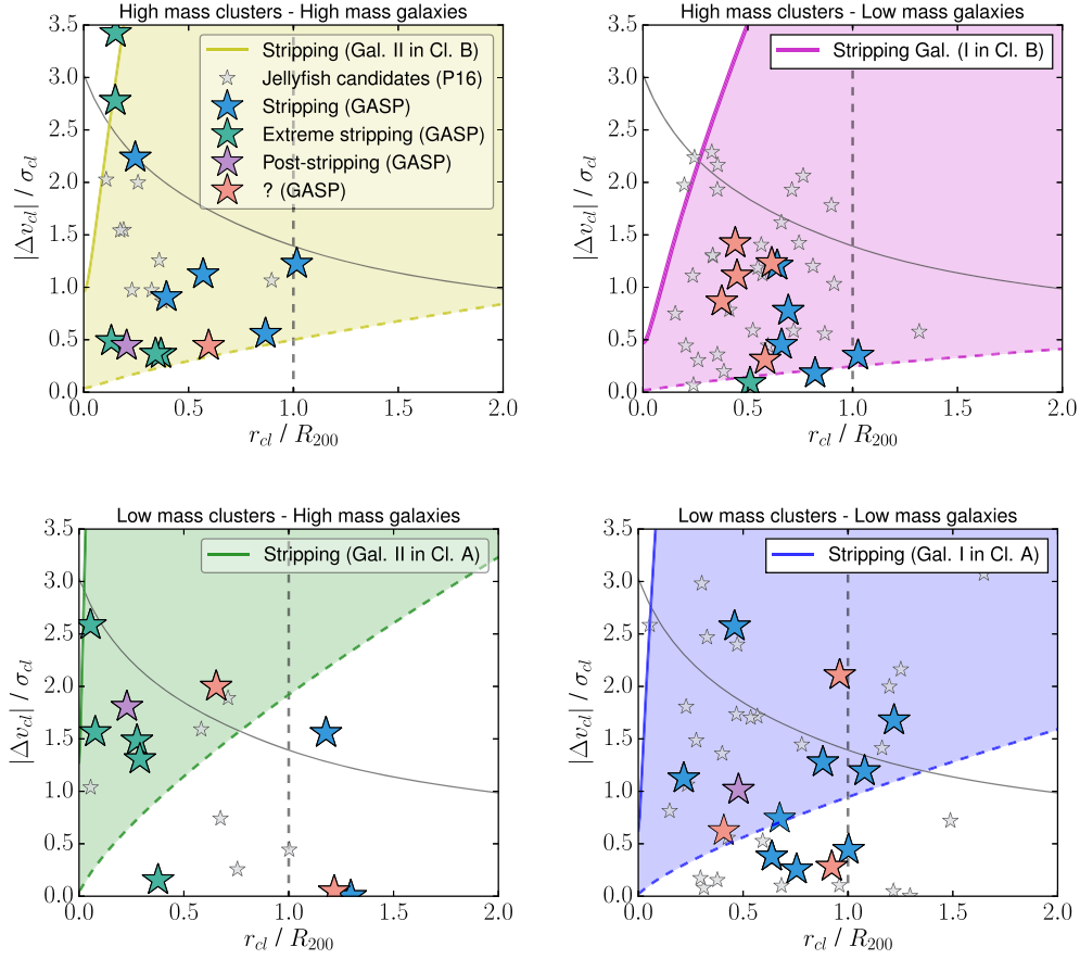
Figure 6. Replaces Fig. 8 of the original paper (coloured areas broadened towards the right of each plot). The location in position versus velocity phase-space of jellyfish galaxies in high mass clusters (top panels; \sigma_{cl} > 750 \text{ km/s} ) and low mass clusters (bottom panels; \sigma_{cl} < 750 \text{ km/s} ) separated in two bins of stellar mass: > 5 \times 10^9 M_\odot (left panels) and < 5 \times 10^9 M_\odot (right panels). Grey stars correspond to the jellyfish sample of P16 while the bigger stars are the confirmed jellyfish galaxies from GASP. Lines of different intensities of ram-pressure are indicated in each case: the dashed coloured lines indicate mild stripping of the gas ( t_r = 4 \times R_d ), while the solid line corresponds to total (100 per cent) stripping. The grey curve corresponds to the escape velocity in a NFW halo. The vertical dashed line indicates r = R_{200} , which is roughly the extent to which all clusters used have a high spectroscopic completeness.
