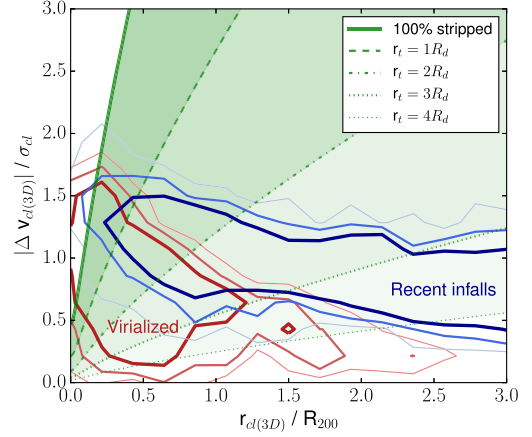
Figure 5. Replaces Fig. 6 of the original paper (green area broadened towards the right of the plot). Position versus velocity phase-space diagram of 15 simulated group and cluster galaxies (mass range from 0.5 \times 10^{13} to 1 \times 10^{15} M_\odot ) from Rhee et al. (2017, private communication; using the YZICS simulations by Choi & Yi (2017)), considering multiple lines of sight, separated into ‘virialized’ (entered the cluster >4 Gyr ago; red contours) and ‘Recent infalls’ (falling towards the cluster for the first time or recently entered the cluster <2 Gyr; blue contours). A galaxy is considered to enter the cluster when it has crossed R_{200} for the first time. The contours enclose 1000, 2500, and 5000 particles from lighter to darker colours respectively. The axes have been normalized by cluster size ( R_{200} ) and cluster velocity dispersion ( \sigma_{cl} ) to allow the stacking of different clusters. The green area indicates the increasing effect of ram-pressure stripping by the ICM in the case of a low-mass galaxy (model galaxy I) falling in a massive cluster (model cluster B). The green lines correspond to different truncation radius ( r_t ) in units of stellar disk scale length ( R_d ). For details see Section 3, and Tables 1 and 2 of the original paper.
