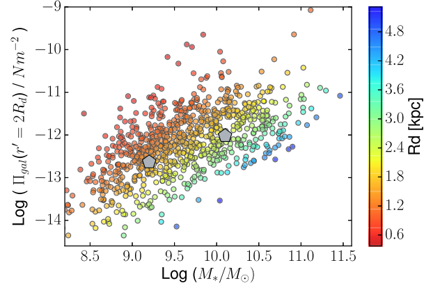
Figure 4. Replaces Fig. 5 in the original paper (almost identical). The anchoring force at r' = 2 \times R_d as a function of stellar mass for all spiral galaxies in our (cluster plus field) sample, colour-coded by R_d . The pentagons correspond to the model galaxies I and II.
