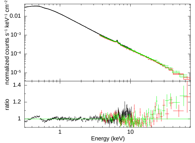
Fig. C.1. Fit over the 0.3–79 keV energy range of the 2014 March 22 XMM-Newton /pn and NuSTAR data with a relativistic reflection baseline model using RELXILL (model \mathcal{A} , n = 10^{19} \text{ cm}^{-3} ).
