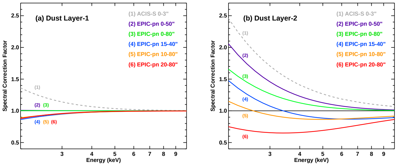
Figure 13. Energy dependent spectral correction factor for the two dust layers for various instruments and spectral extraction regions, based on the best-fit parameters with the COMP-AC-S dust grains (Table 2). Panel-a is for Layer-1 which is local to AX J1745.6-2901; Panel-b is for Layer-2 which is far from AX J1745.6-2901. It is clear that Layer-2 introduces much bigger spectral biases than Layer-1.
